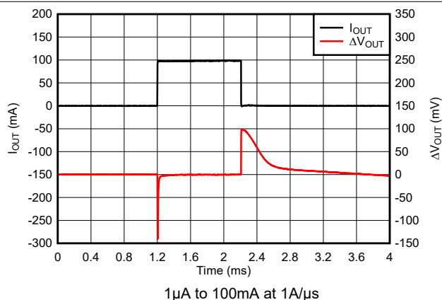
Figure 7-15. TPS76933 Load Transient Response (New Chip)
