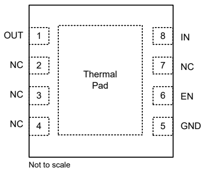
Figure 5-5. DRB Package (Fixed) B Version, 8-Pin VSON, Top View
