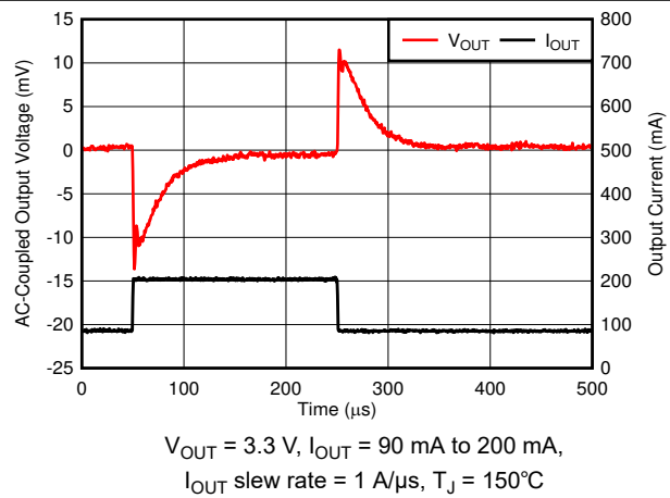
Figure 6-64. Load Transient
