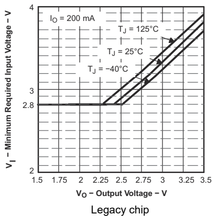
Figure 5-33. Minimum Required Input Voltage vs Output Voltage
