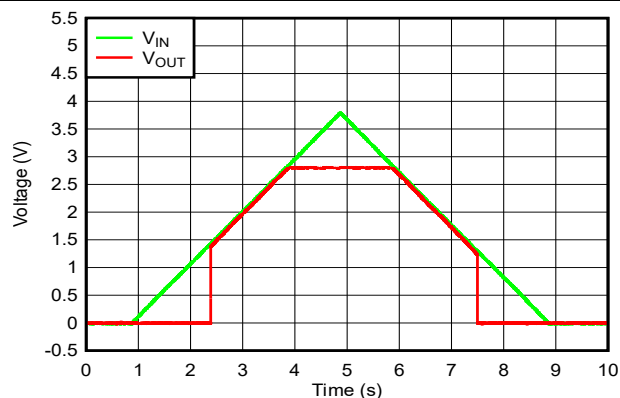
Figure 6-28. TPS794 POWER-UP/POWER-DOWN
