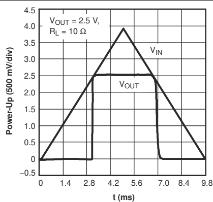
Figure 6-27. TPS794 Power-up/Power-down
