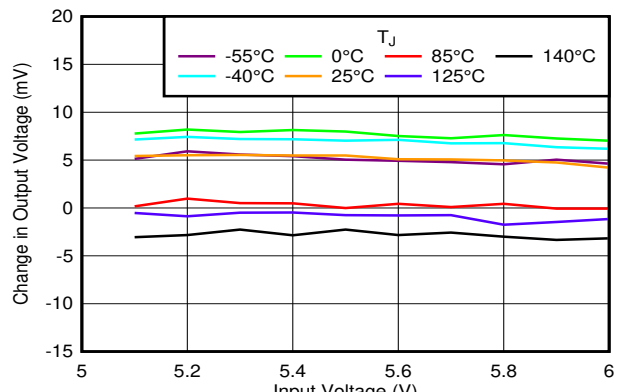
Figure 6-26. Output Accuracy vs V_{IN} and Temperature
