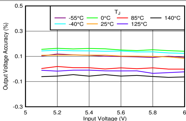
Figure 6-29. Output Accuracy vs V_{IN} and Temperature
