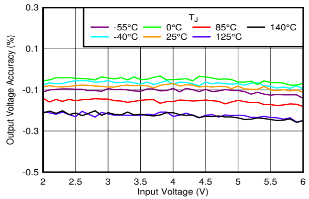
Figure 6-26. Output Accuracy vs V_{IN} and Temperature
