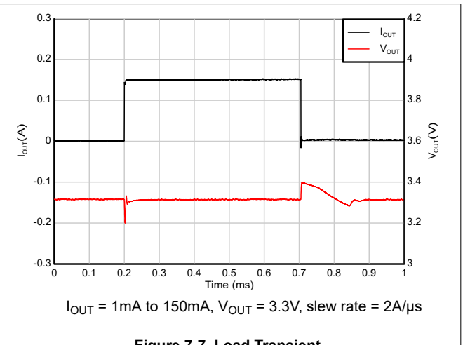
Figure 7-7. Load Transient
