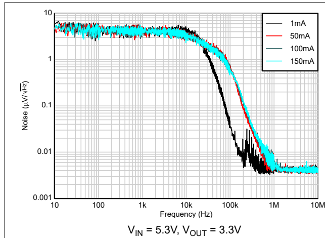
Figure 5-25. Output Noise vs Frequency, Output Current
