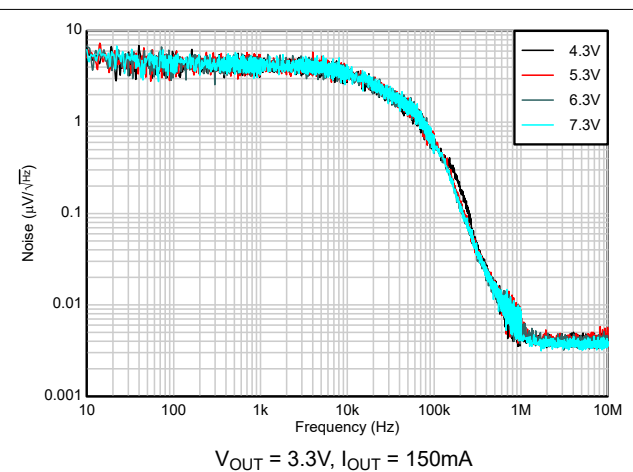
Figure 5-24. Output Noise vs Frequency, Input Voltage
