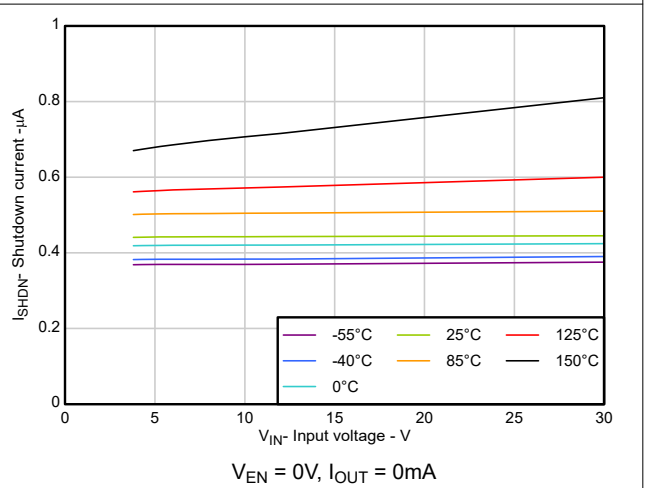
Figure 5-14. Shutdown Current vs Input Voltage
