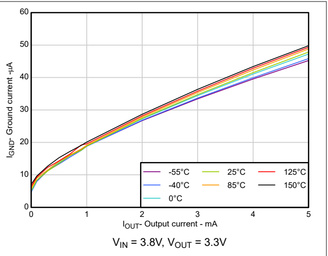
Figure 5-12. Ground Current vs Output Current
