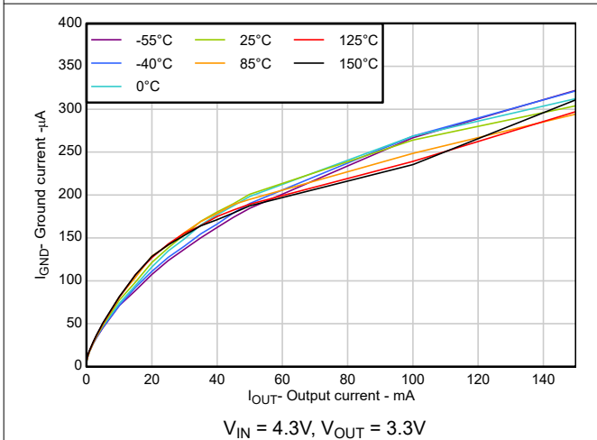
Figure 5-13. Ground Current vs Output Current
