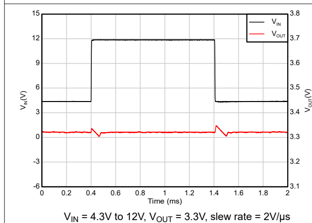
Figure 5-29. Line Transient
