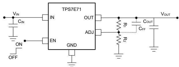
Typical Application
