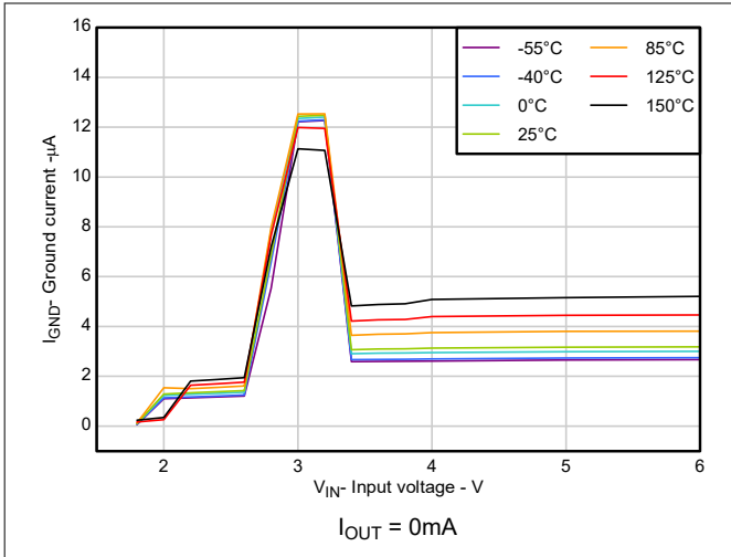
Figure 5-11. Ground Current vs Input Voltage
