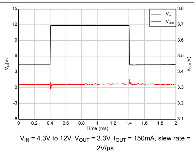
Figure 5-30. Line Transient
