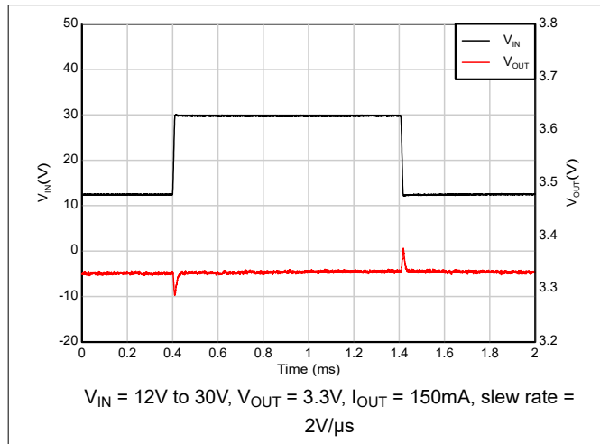
Figure 7-6. Line Transient
