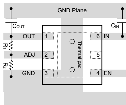
Figure 7-12. Example Layout for TPS7E71, DRV Package
