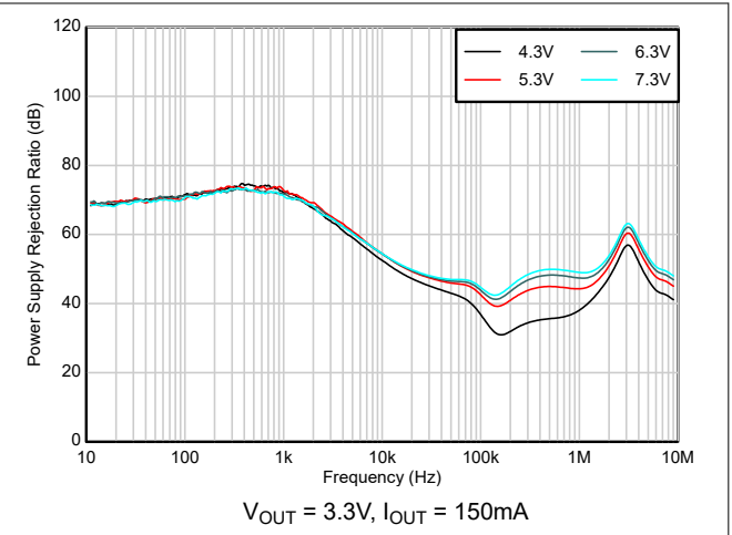
Figure 5-20. Ripple Rejection vs Frequency, Input Voltage
