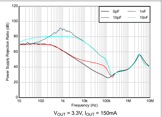
Figure 5-22. Ripple Rejection vs Frequency, C_{FF}
