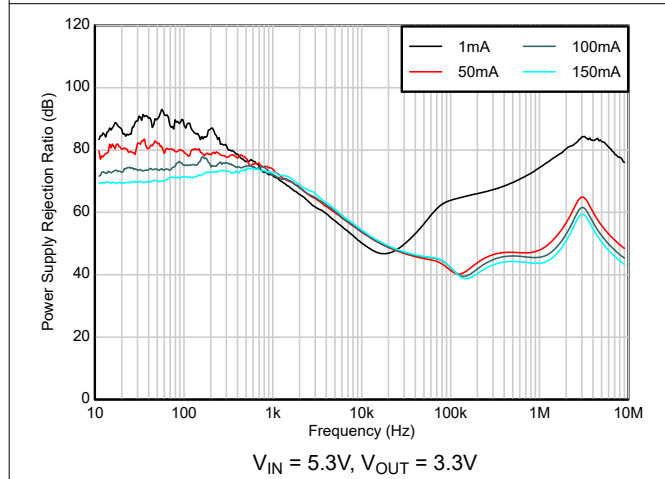
Figure 5-21. Ripple Rejection vs Frequency, Output Current
