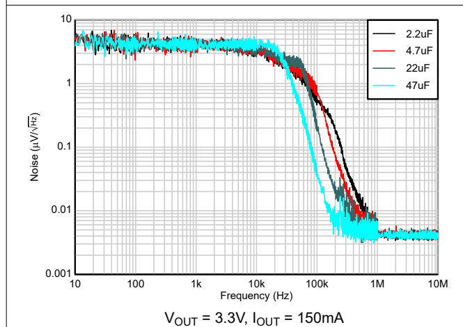
Figure 5-23. Output Noise vs Frequency, C_{OUT}
