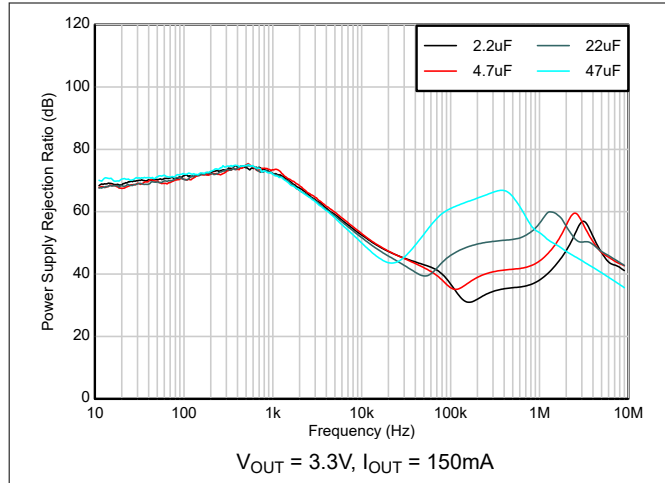
Figure 5-19. Ripple Rejection vs Frequency, C_{OUT}
