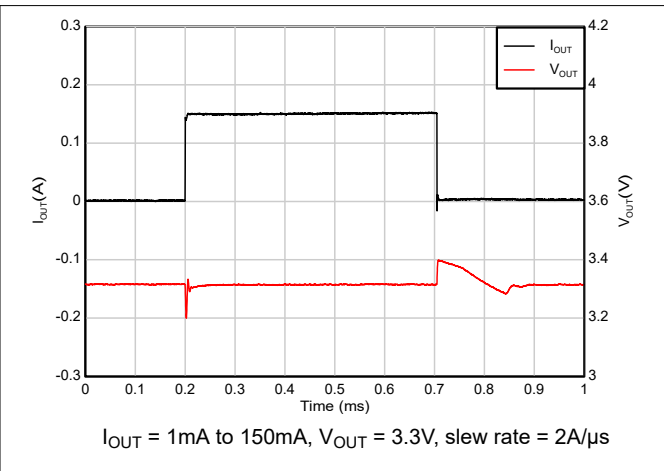
Figure 7-7. Load Transient
