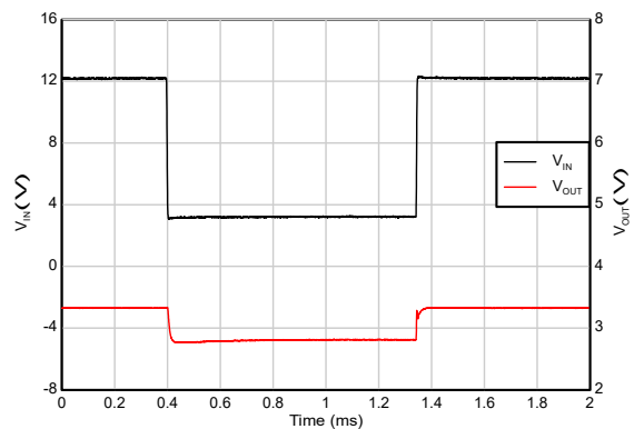
V_{IN} = 12\text{V} to 3\text{V} , V_{OUT} = 3.3\text{V} , I_{OUT} = 100\text{mA} , slew rate = 2\text{V}/\mu\text{s}
