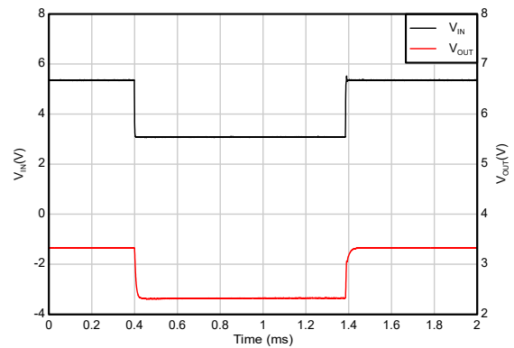
V_{IN} = 5.3\text{V} to 3\text{V} , V_{OUT} = 3.3\text{V} , I_{OUT} = 300\text{mA} , slew rate = 2\text{V}/\mu\text{s}
