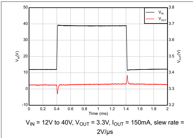
Figure 7-6. Line Transient
