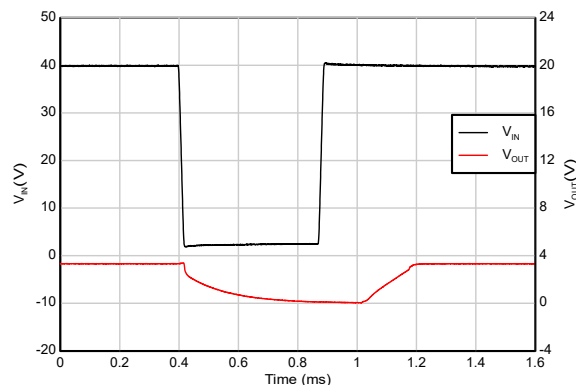
V_{IN} = 40\text{V} to 2\text{V} , V_{OUT} = 3.3\text{V} , I_{OUT} = 50\text{mA} , slew rate = 2\text{V}/\mu\text{s}
