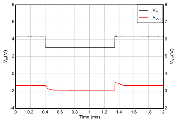
V_{IN} = 4.3\text{V} to 3\text{V} , V_{OUT} = 3.3\text{V} , slew rate = 2\text{V}/\mu\text{s}
