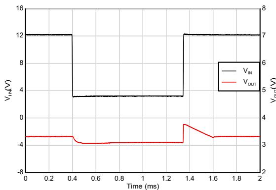
V_{IN} = 12\text{V} to 3\text{V} , V_{OUT} = 3.3\text{V} , slew rate = 2\text{V}/\mu\text{s}
