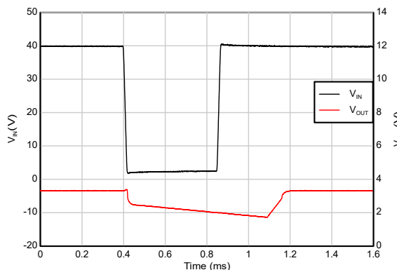
V_{IN} = 40\text{V} to 2\text{V} , V_{OUT} = 3.3\text{V} , slew rate = 2\text{V}/\mu\text{s}
