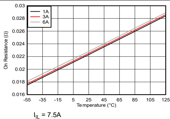
Figure 6-5. On-Resistance vs Temperature Across Loads for HTSSOP at V_{IN} = 5V
