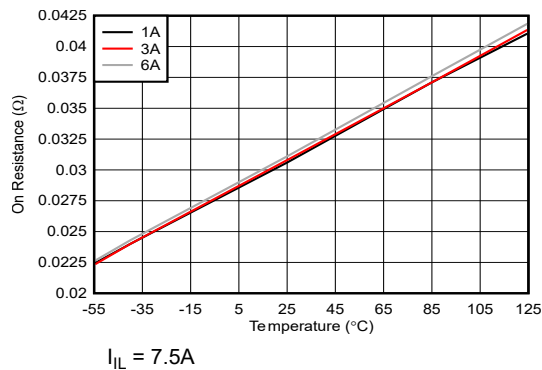
Figure 6-3. On-Resistance vs Temperature Across Loads for CFP and KGD at V_{IN} = 7V
