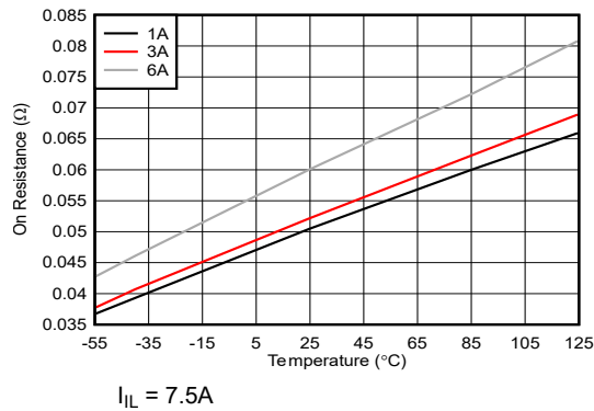
Figure 6-1. On-Resistance vs Temperature Across Loads for CFP and KGD at V_{IN} = 1.5V
