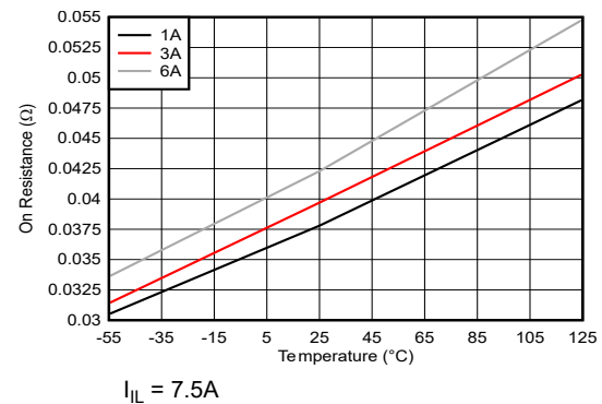
Figure 6-4. On-Resistance vs Temperature Across Loads for HTSSOP at V_{IN} = 1.5V
