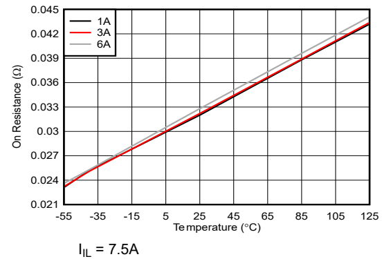
Figure 6-2. On-Resistance vs Temperature Across Loads for CFP and KGD at V_{IN} = 5V
