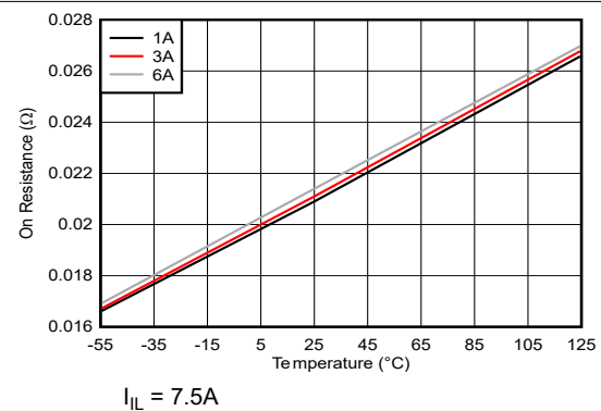
Figure 6-6. On-Resistance vs Temperature Across Loads for HTSSOP at V_{IN} = 7V
