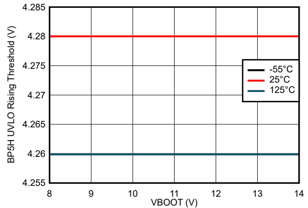
Figure 7-22. BP5H UVLO Rising Threshold vs BOOT Voltage
