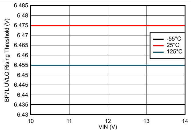
Figure 7-24. BP7L UVLO Rising Threshold vs VIN Voltage
