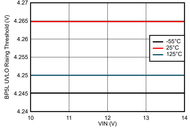
Figure 7-20. BP5L UVLO Rising Threshold vs VIN Voltage
