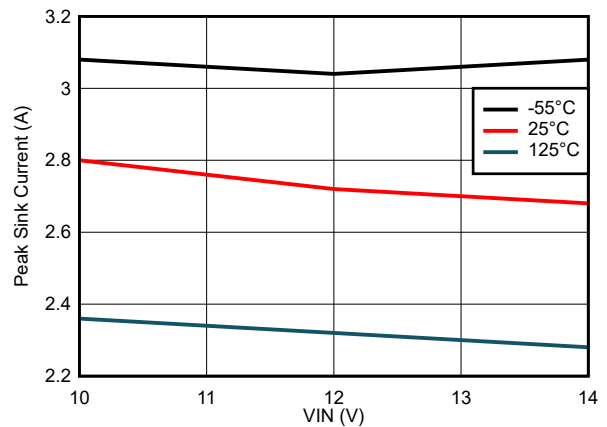
Figure 7-10. Peak Sink Current vs VIN Voltage
