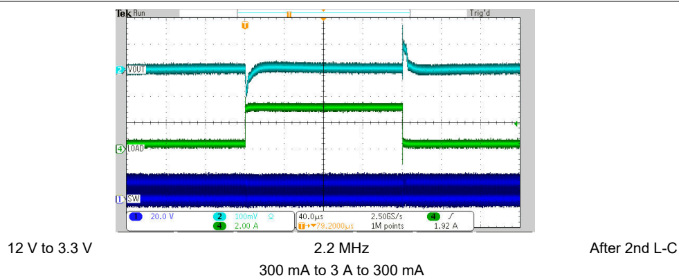
Figure 8-14. Load Transient
