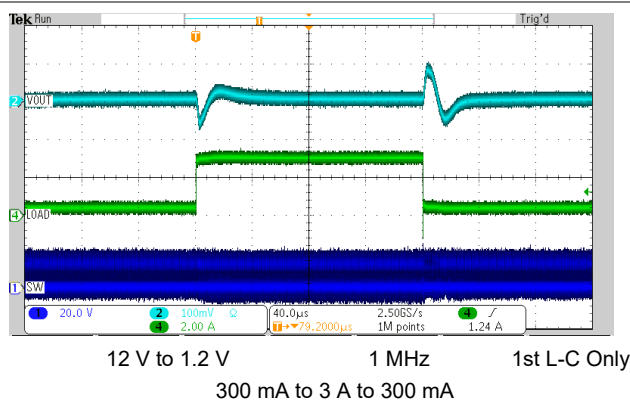
Figure 8-9. Load Transient
