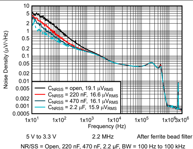
Figure 6-32. Output Noise Density vs Frequency
