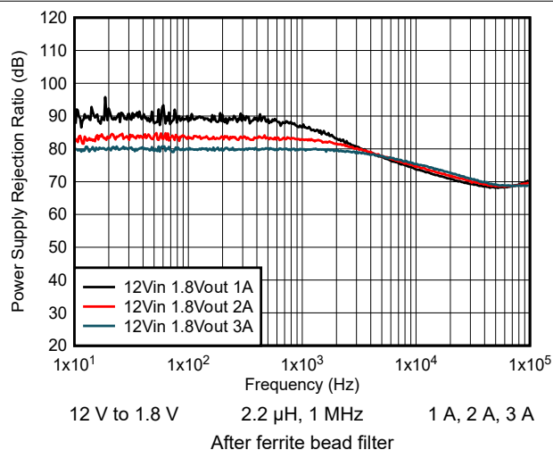
Figure 6-34. PSRR vs Frequency
