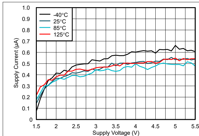
Figure 5-2. Supply Current vs Supply Voltage
