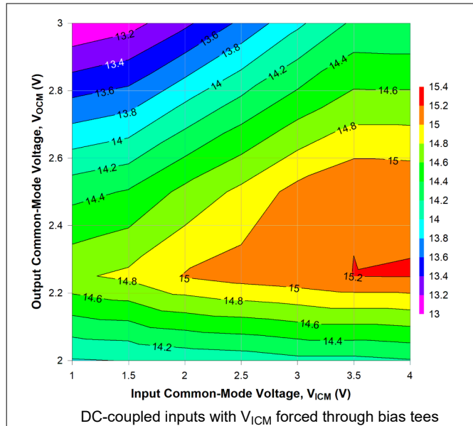
Figure 6-41. OP1dB Across V_{\text{ICM}} and V_{\text{OCM}} at 500MHz
