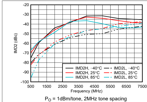
Figure 6-75. IMD2 Across Temperature
