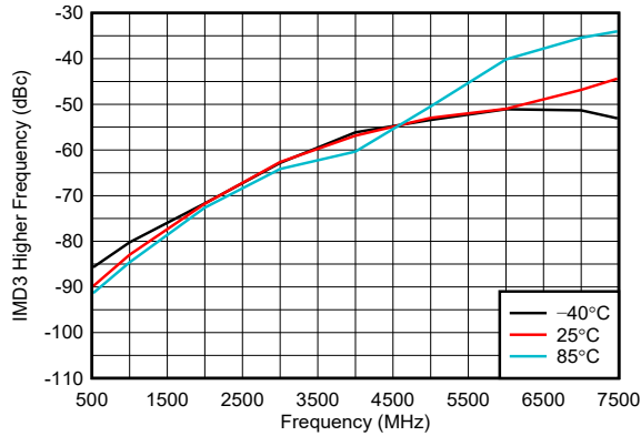
Figure 6-69. IMD3 Higher Across Temperature
