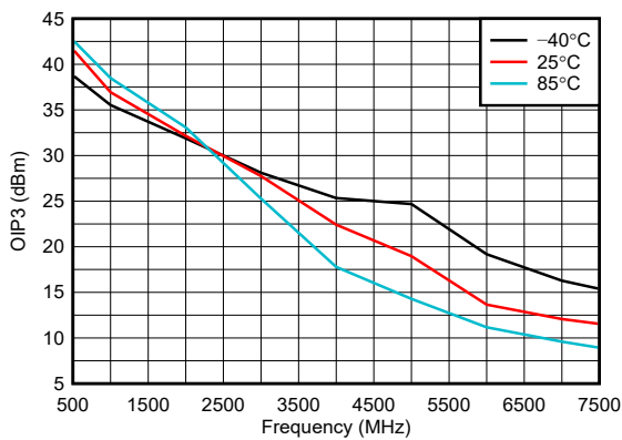
Figure 6-59. OIP3 Across Temperature
