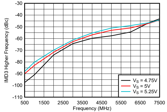
Figure 6-70. IMD3 Higher Across Supply Voltage
