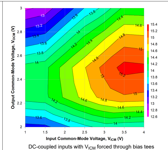
Figure 6-42. OP1dB Across V_{\text{ICM}} and V_{\text{OCM}} at 2GHz
