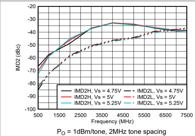
Figure 6-76. IMD2 Across Supply Voltage
