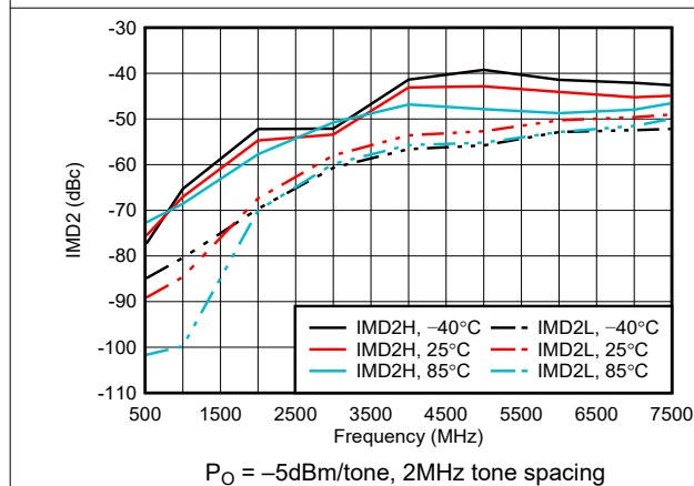
Figure 6-77. IMD2 Across Temperature
