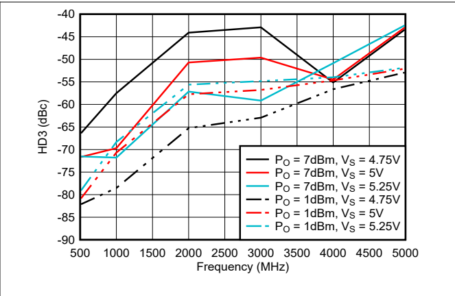
Figure 6-82. HD3 Across Output Power and Supply Voltage
