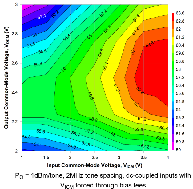
Figure 6-40. OIP2 Across V_{ICM} and V_{OCM} at 2GHz
