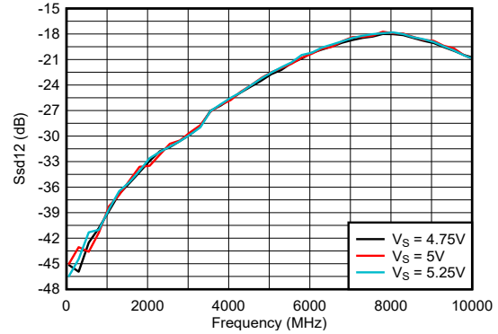
Figure 6-58. Reverse Isolation (Ssd12) Across Supply Voltage
