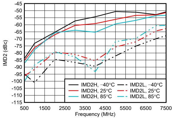
Figure 6-25. IMD2 Across Temperature
