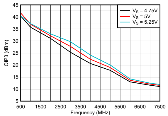
Figure 6-60. OIP3 Across Supply Voltage
