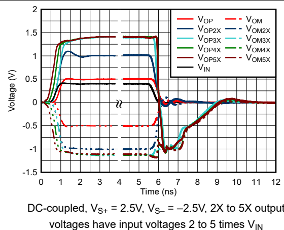
Figure 6-92. Overdrive Recovery Response
