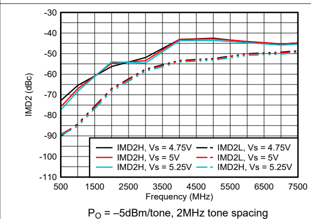
Figure 6-78. IMD2 Across Supply Voltage
