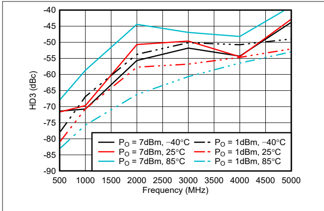
Figure 6-81. HD3 Across Output Power and Temperature
