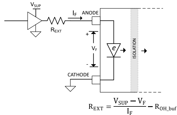
Figure 7-2. Driving the Input Stage with One Buffer and Anode Resistor
