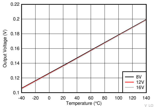
Figure 6-13. LO High Output Voltage ( V_{LOH} ) I_O=-100mA
