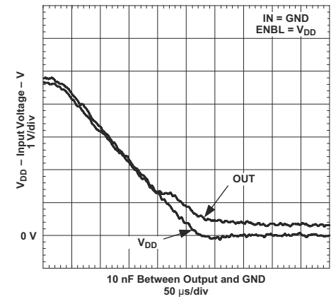
Figure 7-20. Output Behavior vs V_{DD} (UCC27321)
