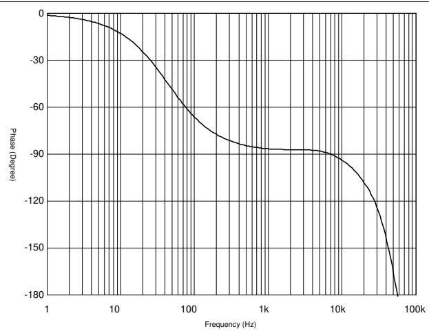
Figure 8-3. Converter Open Loop Bode Plot - Phase
