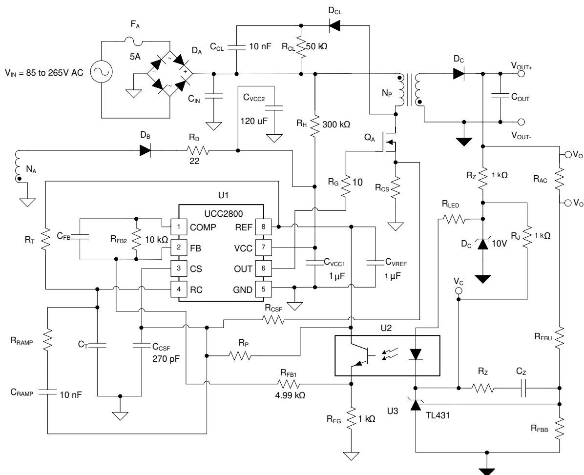
Figure 8-1. Typical Application Circuit
