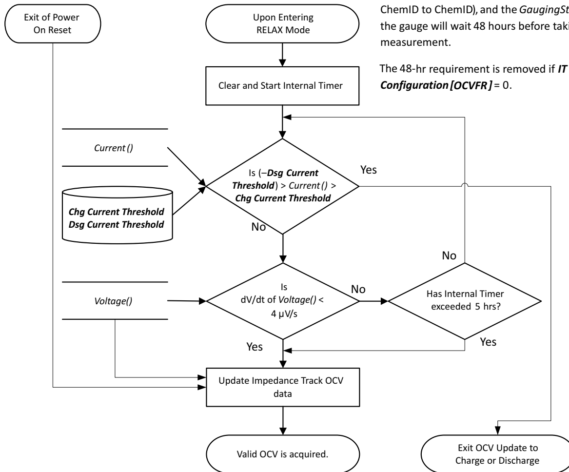
Figure 7-2. OCV Measurement
