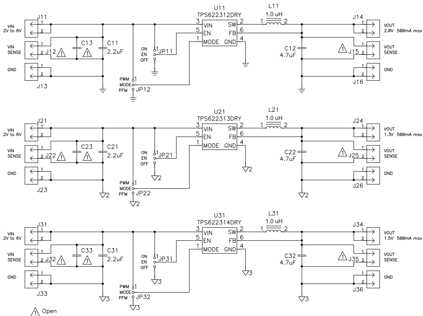
Figure 4. TPS622312/13/14EVM-574 Schematic
