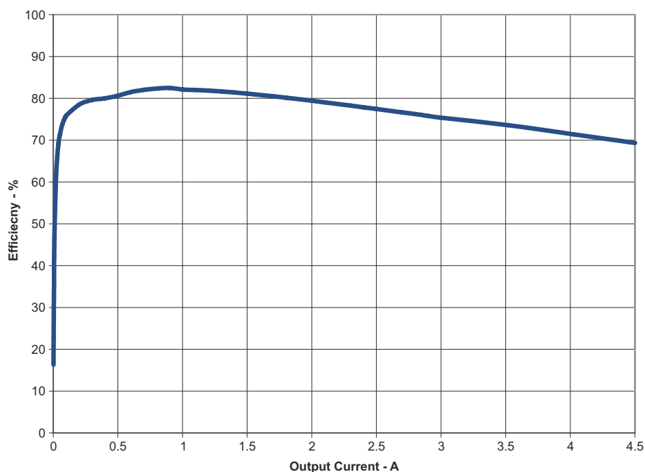
Figure 4-1. TPS54429EVM-608 Efficiency
