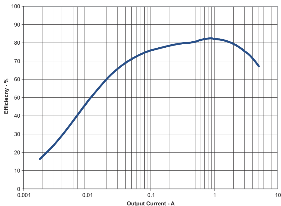
Figure 4-2. TPS54429EVM-608 Light Load Efficiency
