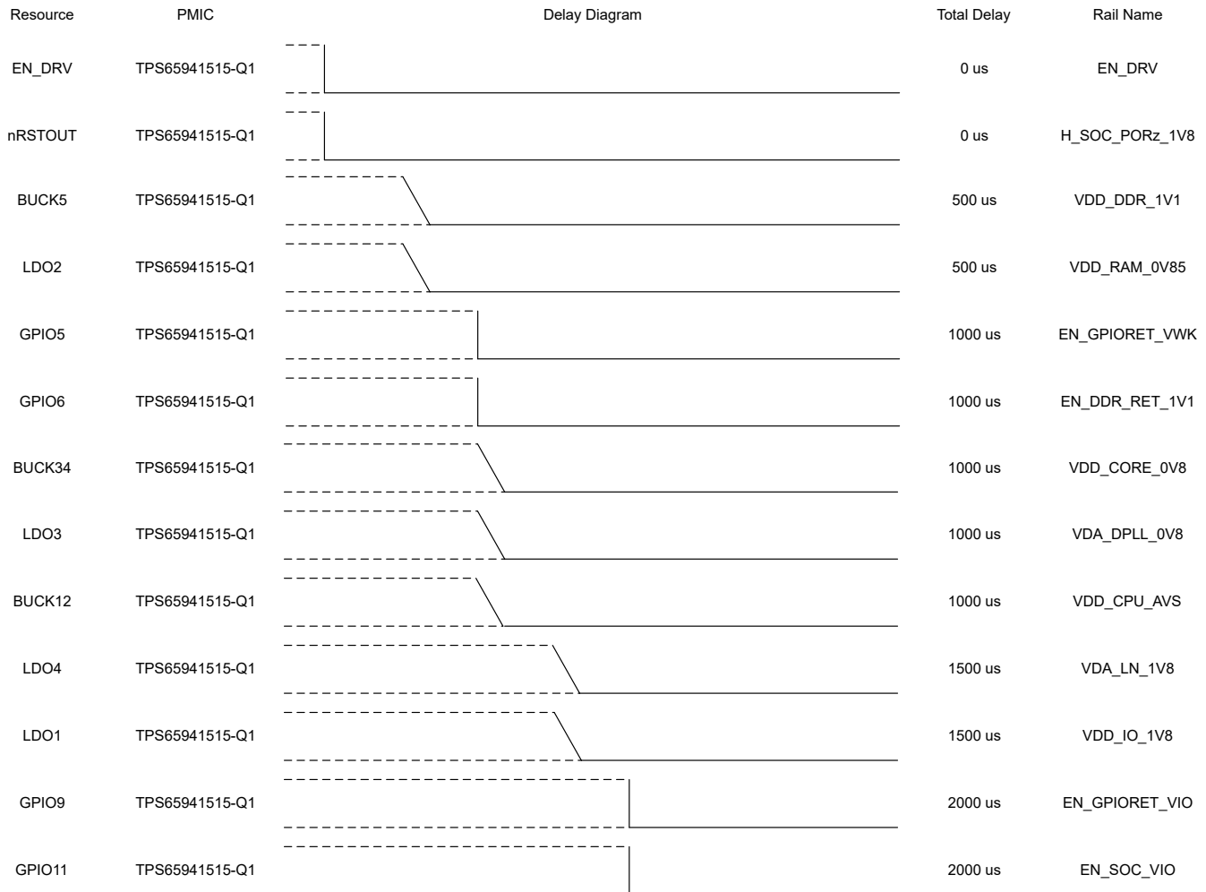
Figure 6-3. TO_SAFE_ORDERLY and TO_STANDBY Power Sequence
