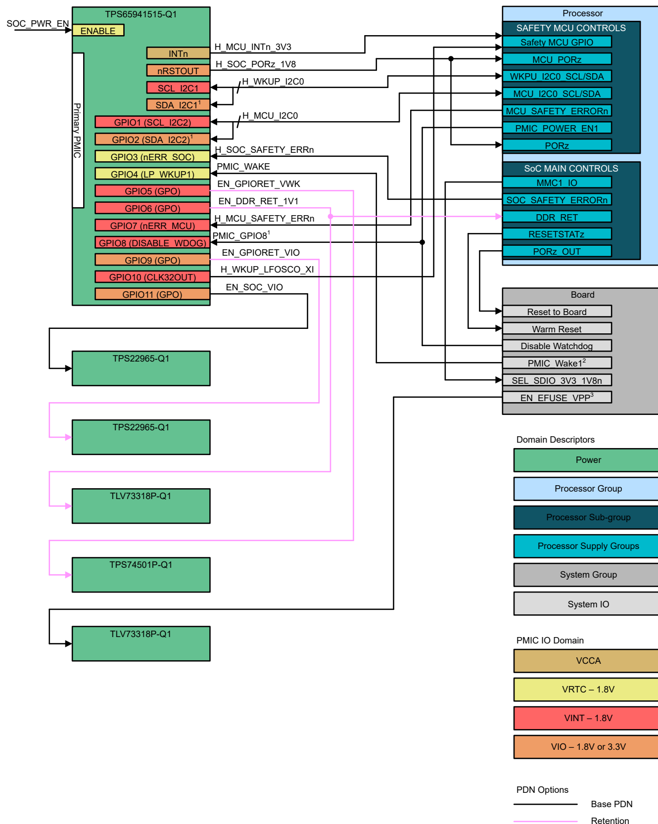
Figure 3-2. TPS65941515-Q1 Digital Connections
