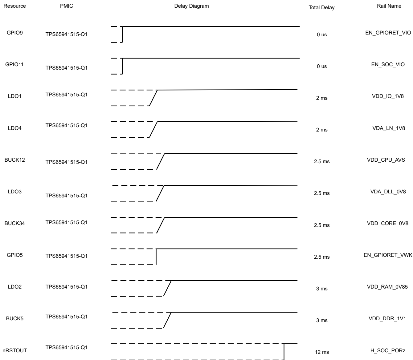
Figure 6-5. TO_ACTIVE Sequence
