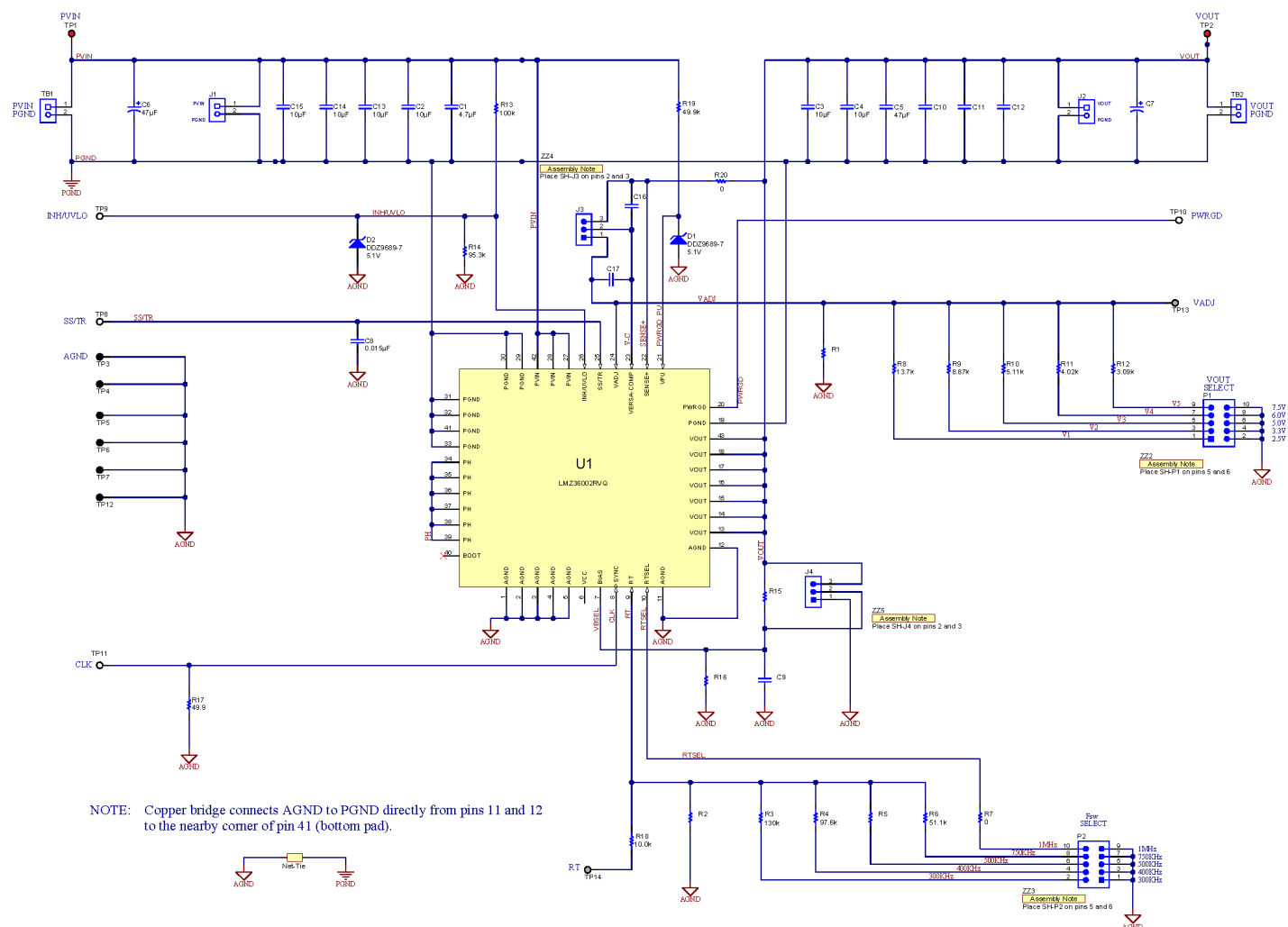
Figure 8. LMZ36002EVM Schematic
