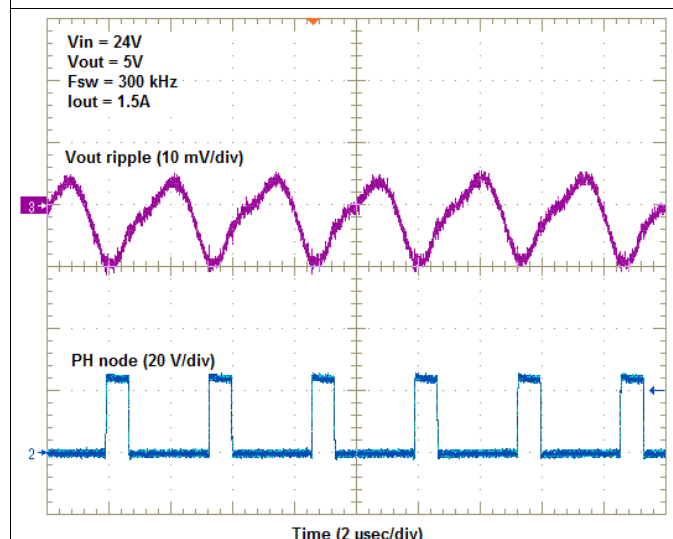
Figure 4. LMZ36002EVM Ripple Voltage (Fsw = 300 KHz)
