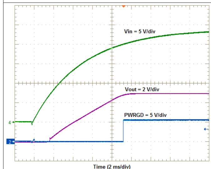
Figure 6. LMZ36002EVM Start-up Waveforms
