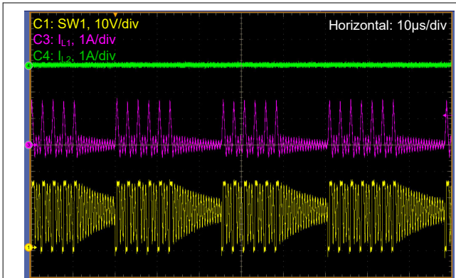
Figure 3-4. V_{in} = 14.4V , V_{out} = 24V , DEM, I_{load} = 0.1A
