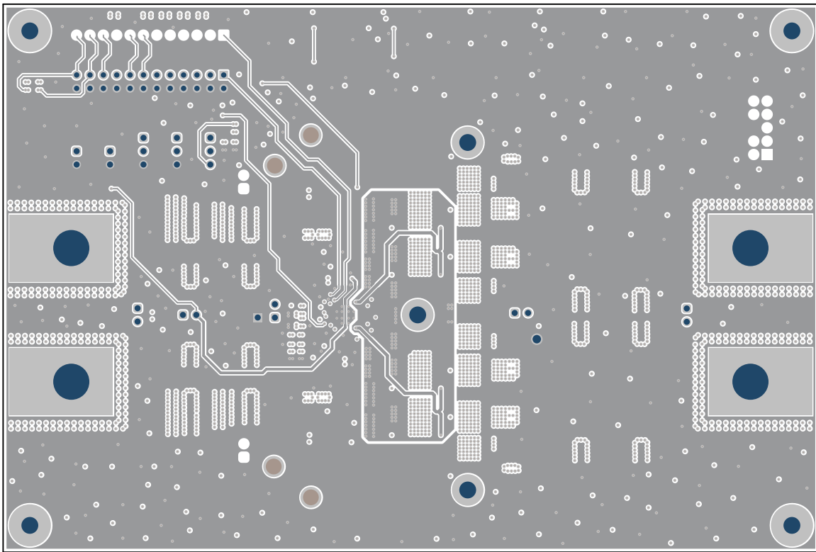
Figure 4-8. Signal Layer 4
