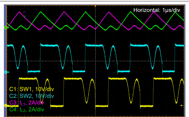
Figure 3-5. V_{in} = 14.4V , V_{out} = 24V , DEM, I_{load} = 1A
