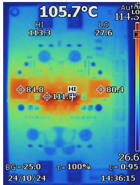
Figure 3-11. V_{in} = 14.4V , V_{out} = 45V , P_{OUT} = 300W , Natural Convection
