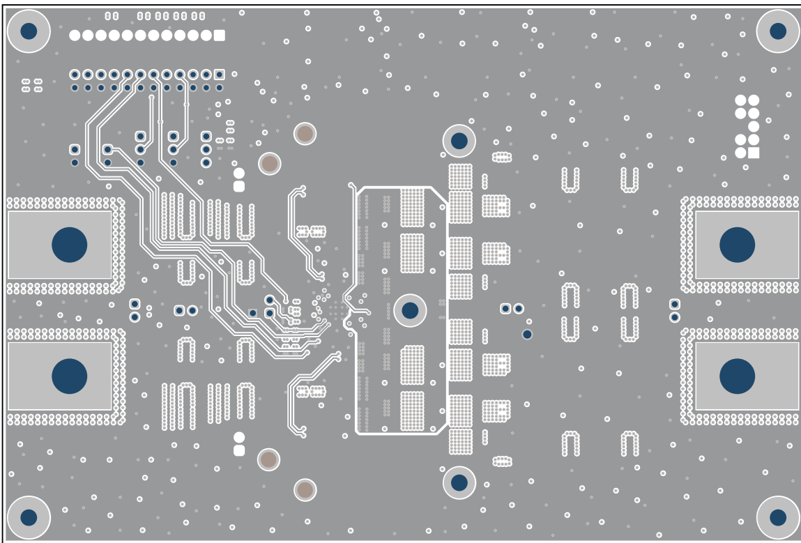
Figure 4-7. Signal Layer 3
