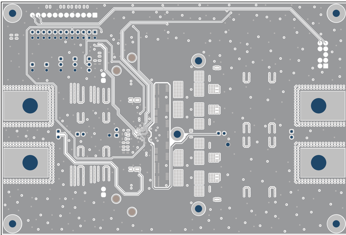
Figure 4-6. Signal Layer 2
