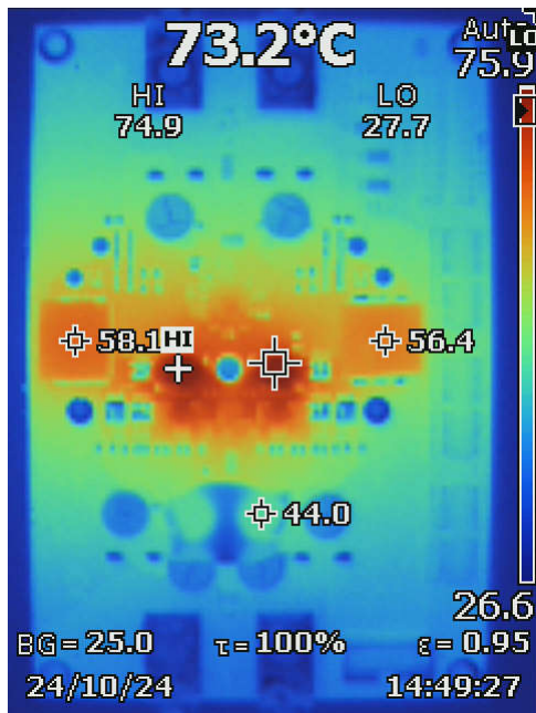
Figure 3-10. V_{in} = 14.4V , V_{out} = 24V , P_{OUT} = 300W , Natural Convection
