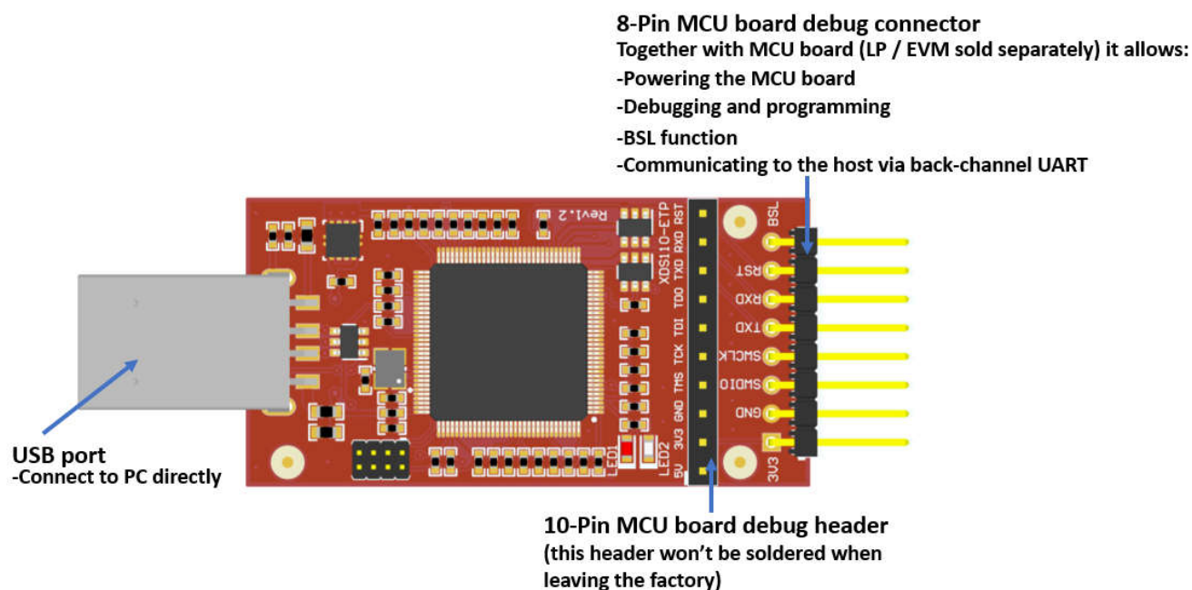
Figure 1-1. XDS110-ETP Overview
