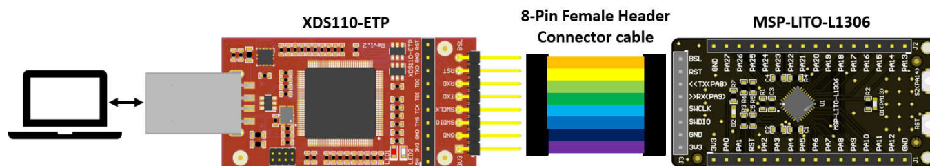
Figure 3-1. Hardware Setup
