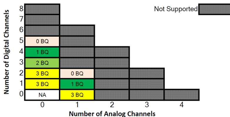
Figure 3-4. Channel Combinations for 192 kHz Linear Phase Filter with AGC/DRE Enabled
