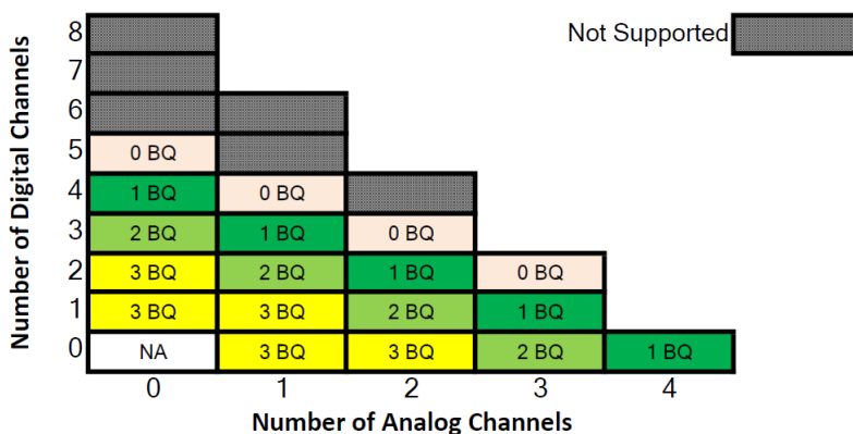
Figure 3-5. Channel Combinations for 192 kHz Linear Phase Filter with AGC/DRE Disabled
