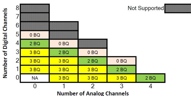
Figure 3-3. Channel Combinations for 96 kHz with DRE/AGC Disabled
