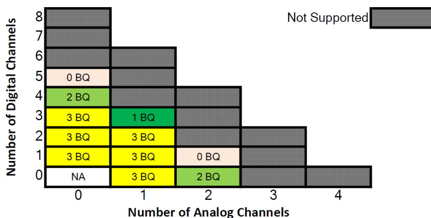
Figure 3-2. Channel Combinations for 96 kHz with DRE/AGC Enabled
