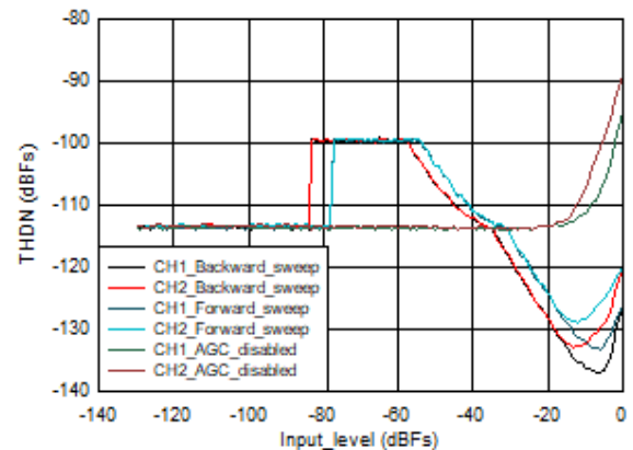
Figure 3-2. THDN vs. Input_Level 48 KHz
