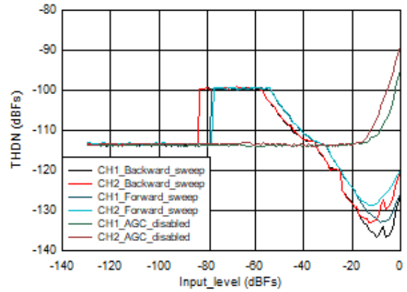
Figure 3-8. THDN vs. Input_Level 48 KHz (Enhanced Mode)
