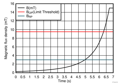
Figure 4. Magnetic Flux Density for End-of-Travel Detection
