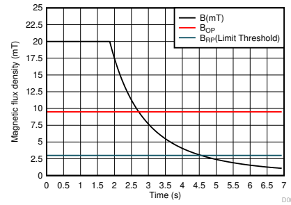
Figure 3. Magnetic Flux Density for Case Tamper Detection
