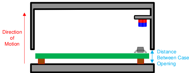
Figure 2. Case Tamper Detection Implementation
