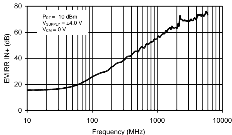
Figure 1. TLV2422 EMIRR IN+ vs Frequency
