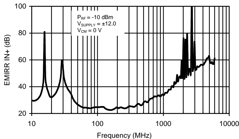
Figure 1. TLE2037 EMIRR IN+ vs Frequency
