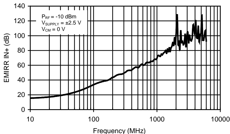
Figure 1. TLV2341 EMIRR IN+ vs Frequency
