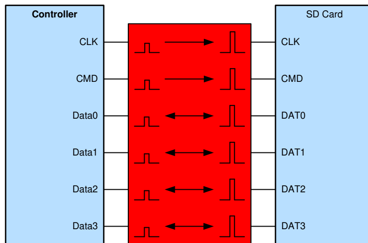
Example of Using Voltage Translation With an SD Card Communication Bus
