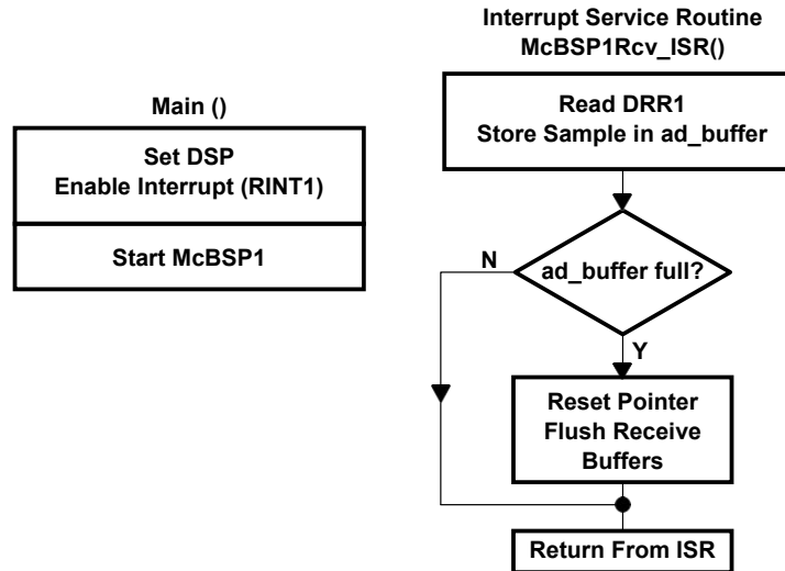
Figure 2. Software Flow Chart
