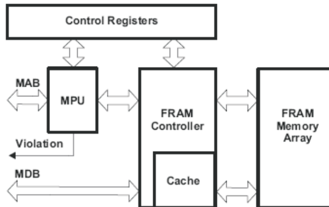
Figure 3. FRAM Controller Block Diagram
