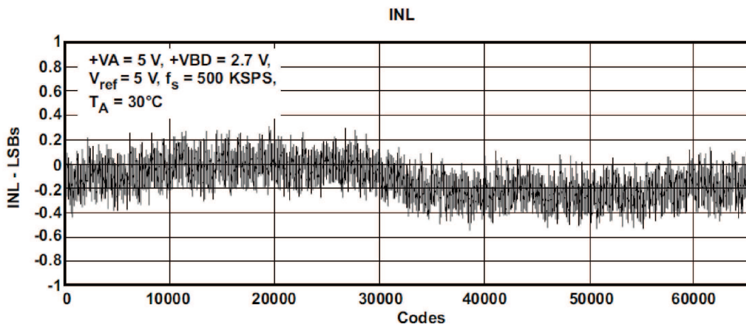
Figure 5. INL
