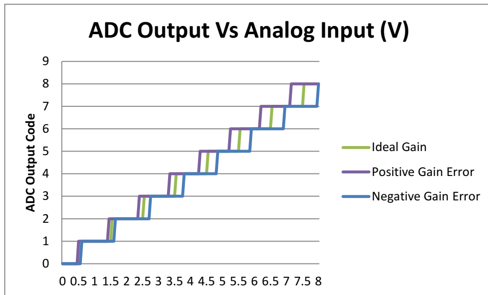
Figure 3. Gain Error
