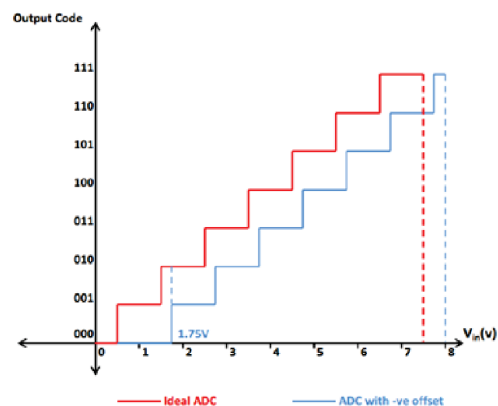
Figure 2. Negative Offset Error
