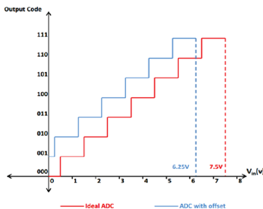
Figure 1. Positive Offset Error
