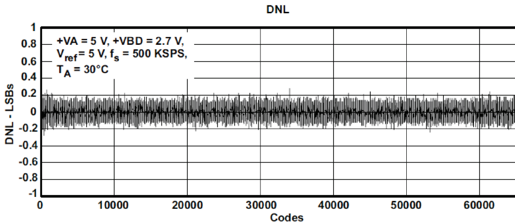
Figure 4. DNL
