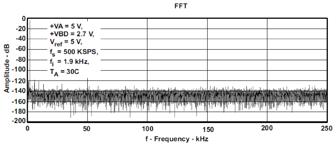
Figure 6. Typical ADC Output Spectrum Plot
