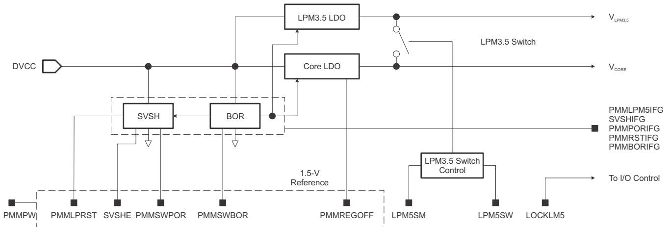
Figure 1. PMM Block Diagram
