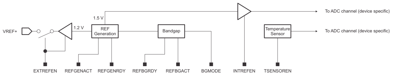
Figure 2. VREF Generation Block Diagram
