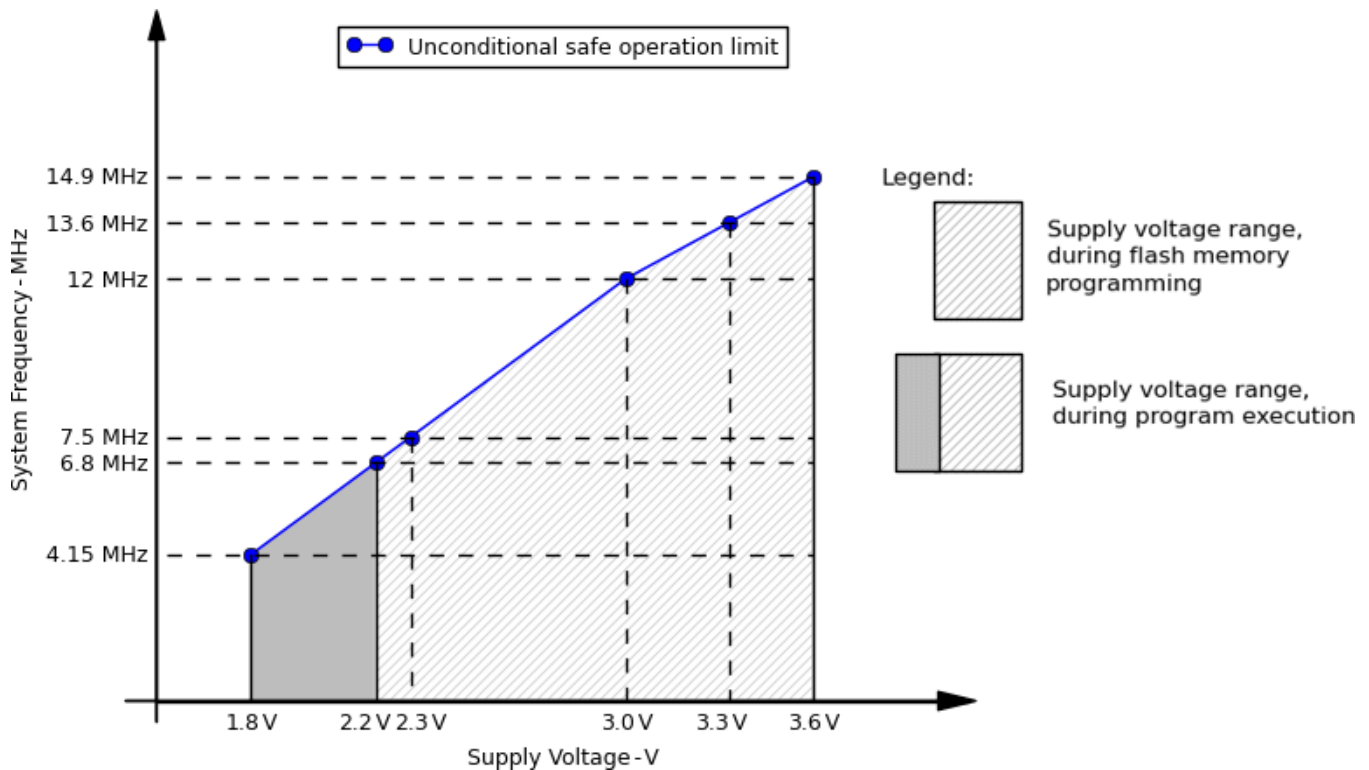
Figure 2. V CC vs Frequency – Safe Operating Conditions for LFXT1 in HF Mode and for Digital External Clock Sources
