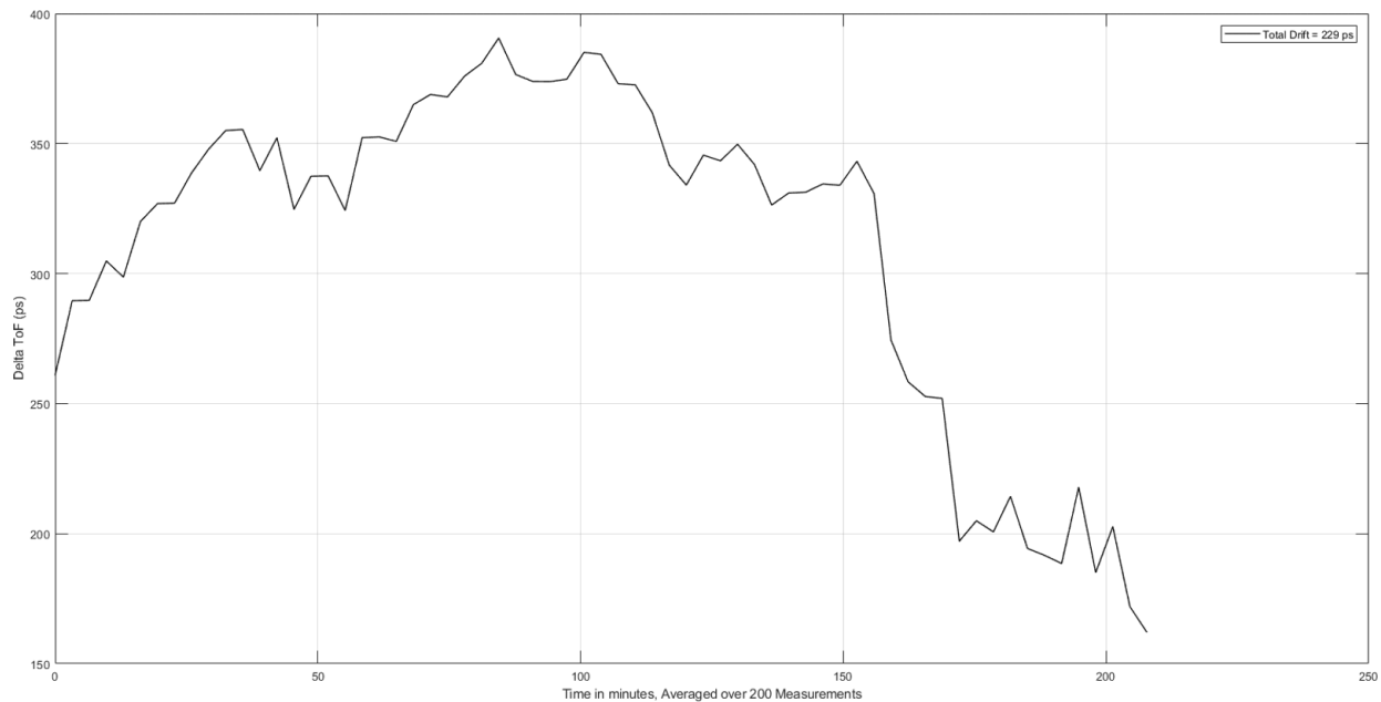
Figure 3. Zero Flow Drift (ZFD) for a Gas Meter Application
