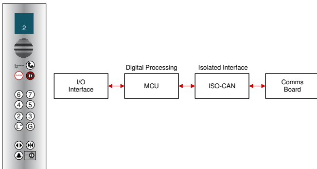
Figure 1. Isolated CAN in Elevators
