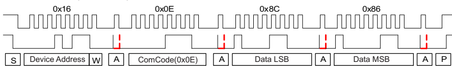
SM Bus Write Word (without PEC)
