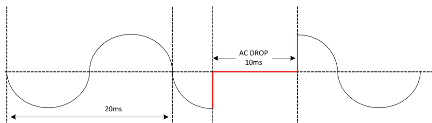
Figure 2. AC Input Voltage Waveform during AC Drop 10 ms at 90°
