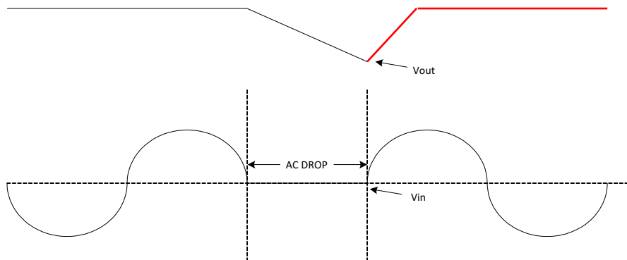
Figure 3. The Typical Waveform of Output Voltage and AC Input Voltage during AC Drop
