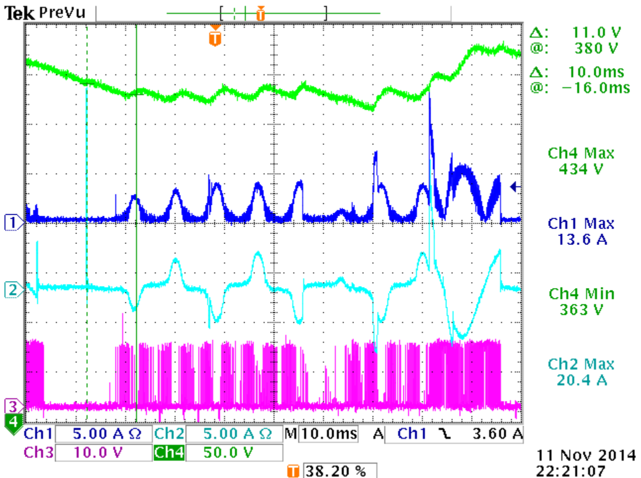
Figure 5. AC Drop Test without Proposed Method
