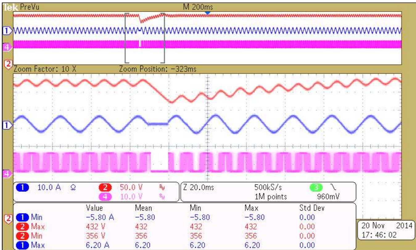
Figure 6. AC Drop Test with Proposal Method
