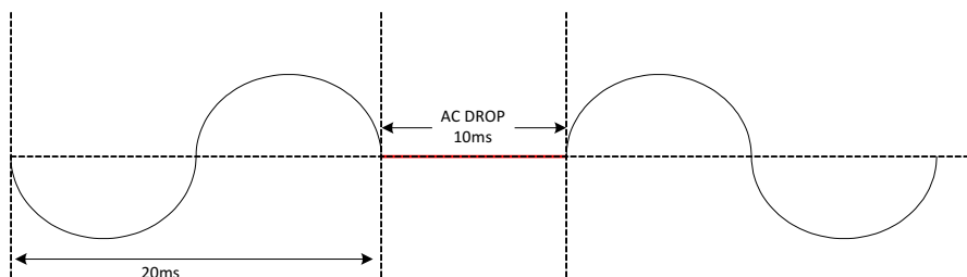
Figure 1. AC Input Voltage Waveform during AC Drop 10 ms at 0°
