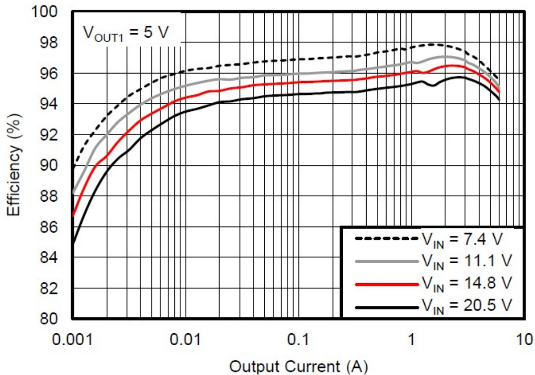
Figure 1. TPS51285A Efficiency Plot
