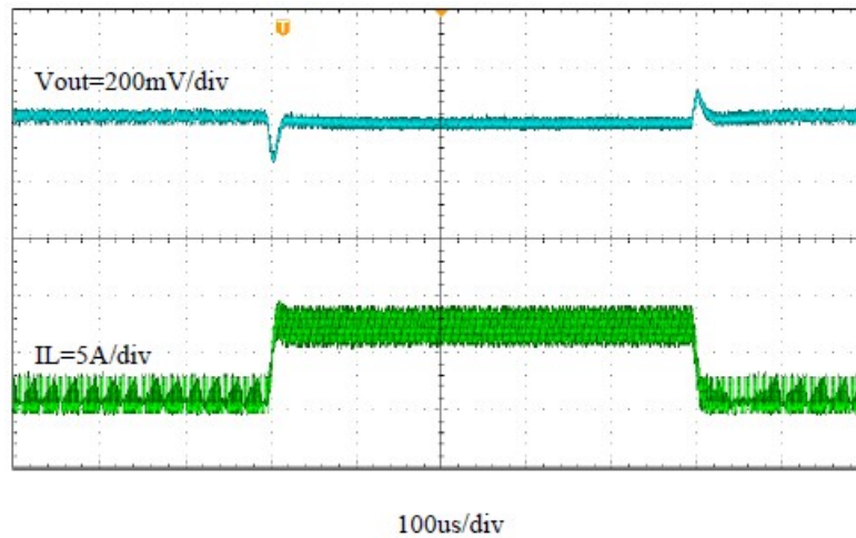
Figure 2. TPS51395 Transient Waveform
