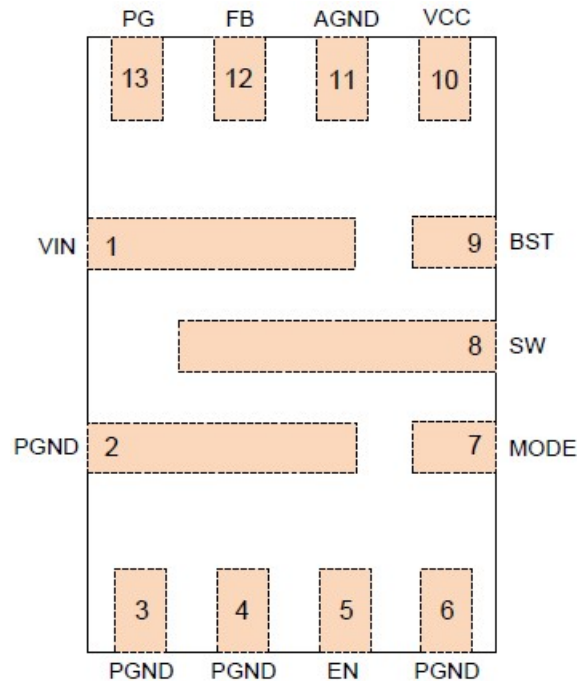
Figure 4. TPS566335 in 2x3mm QFN Package
