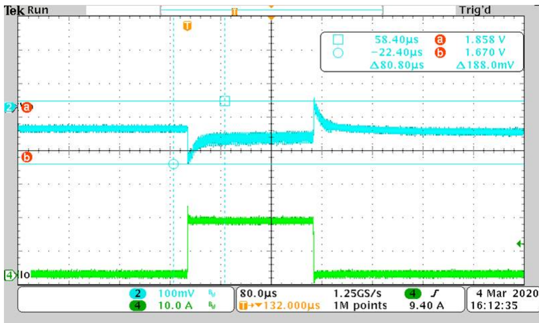
Figure 3. TPS51215A Load Transient Waveform
