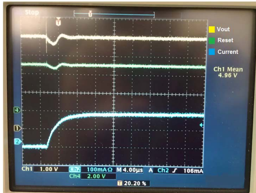
Figure 1. 68 \mu F/16V Nichicon UD Series Cap at V_{IN} = 20V
