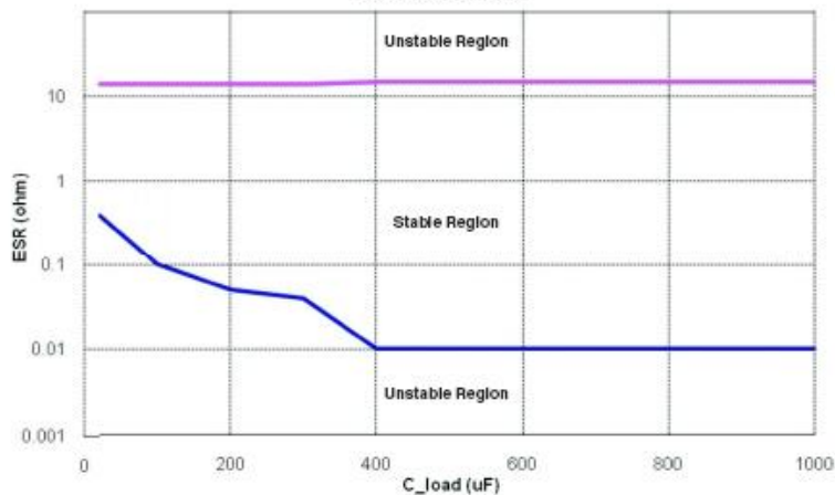
ESR STABILITY vs LOAD CAPACITANCE
