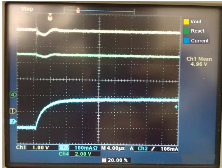
Figure 2. 68 \mu F/16V Panasonic EEE-FT Series Cap at V_{IN} = 20V
