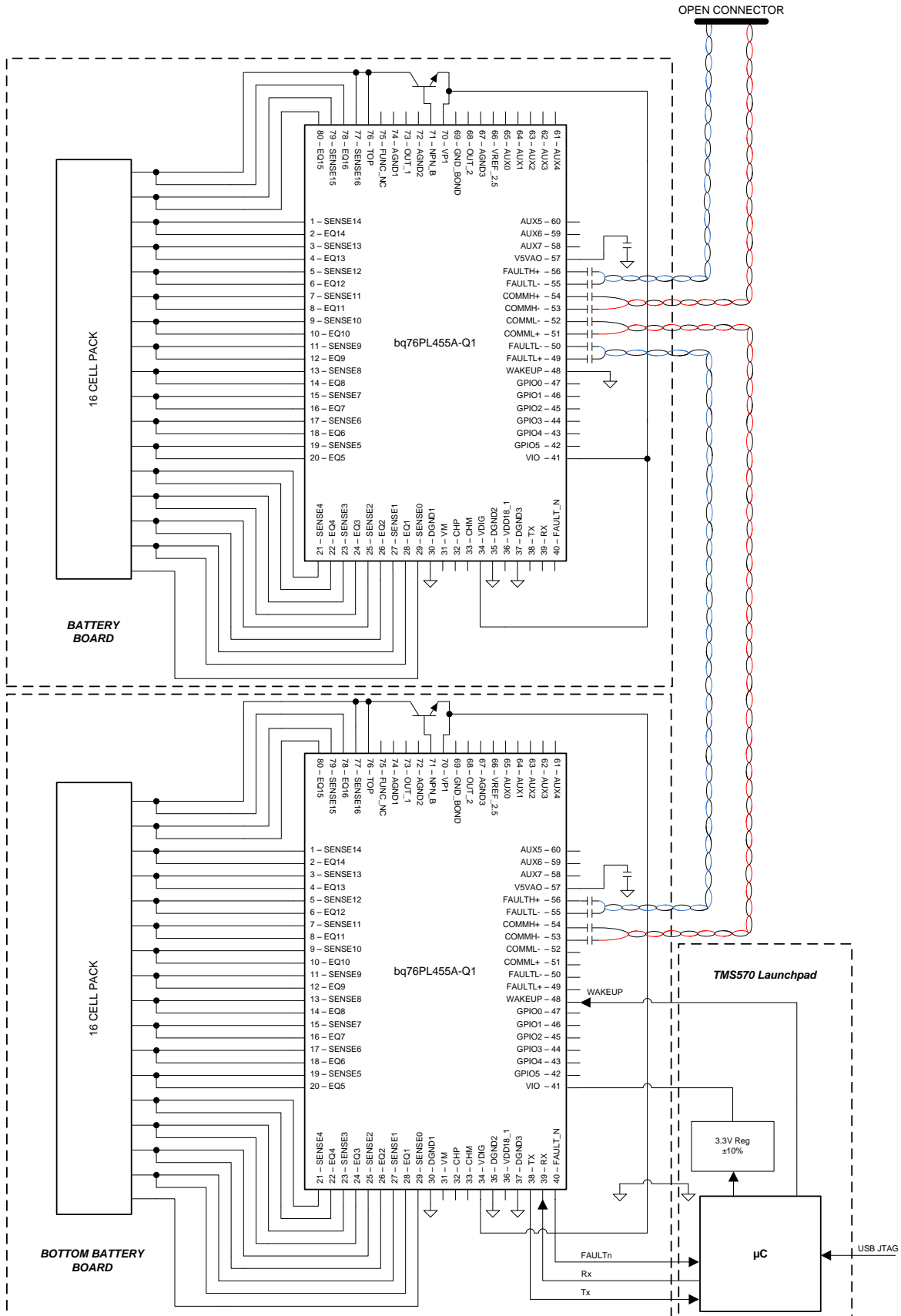
Figure 1. System Block Diagram
