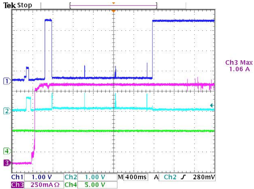
Figure 5. TPS25810 and TPS2544 (CDP Mode) Test With Galaxy S6, With Type C-to-B Dongle Connected to Host Then Plug In Device
