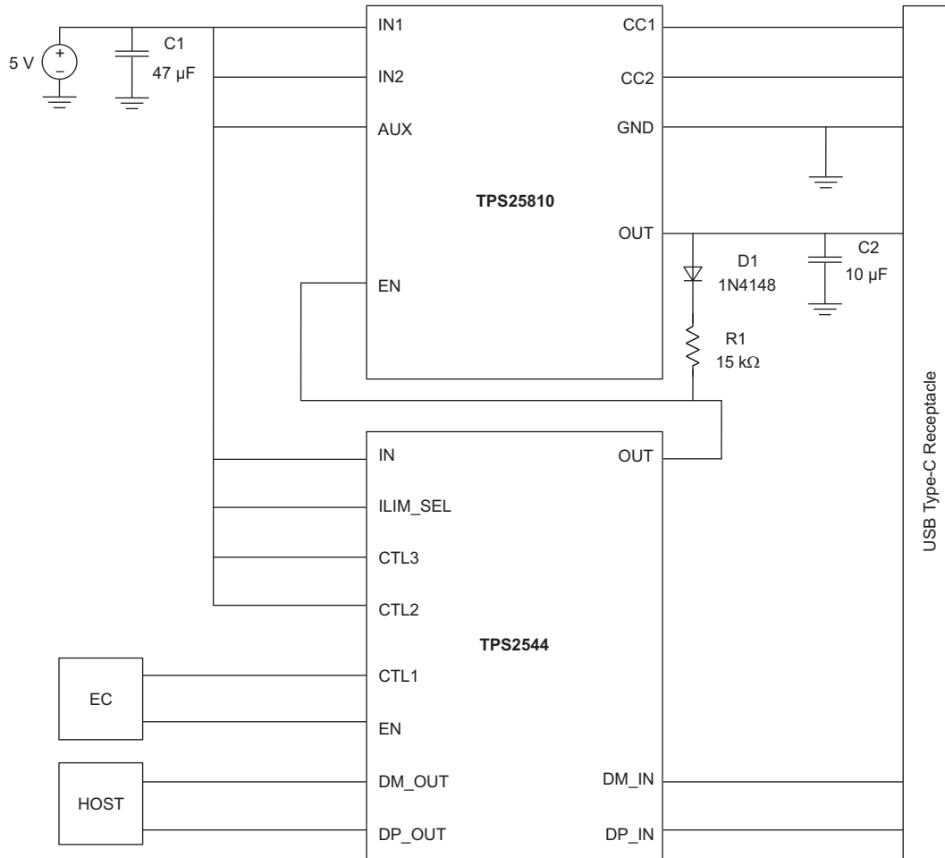
Figure 1. TPS25810 Charging Port Over USB Type-C Circuit Utilizing TPS2544
