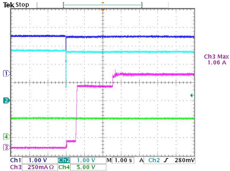
Figure 7. TPS25810 and TPS2544 (DCP Auto Mode) Test With iPhone6, With Type C-to-B Dongle Connected TO Host Then Plug In Device
