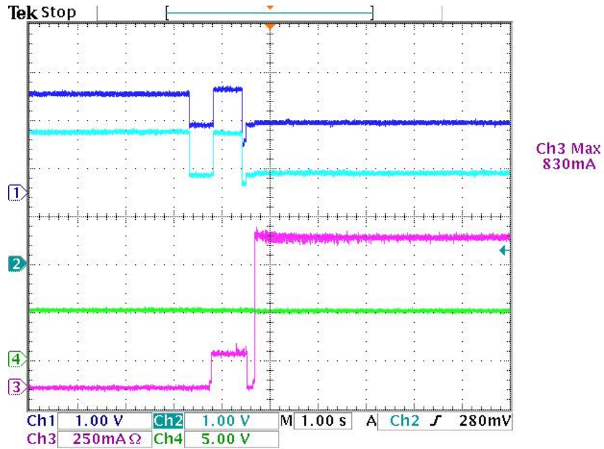
Figure 11. TPS25810 and TPS2544 (DCP Auto Mode) Test With HTC Sense, With Type C-to-B Dongle Connected to Host Then Plug In Device
