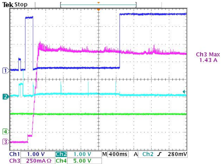
Figure 3. TPS25810 and TPS2544 (CDP Mode) Test With iPhone6, With Type C-to-B Dongle Connected to Host, Then Plug in the Device
