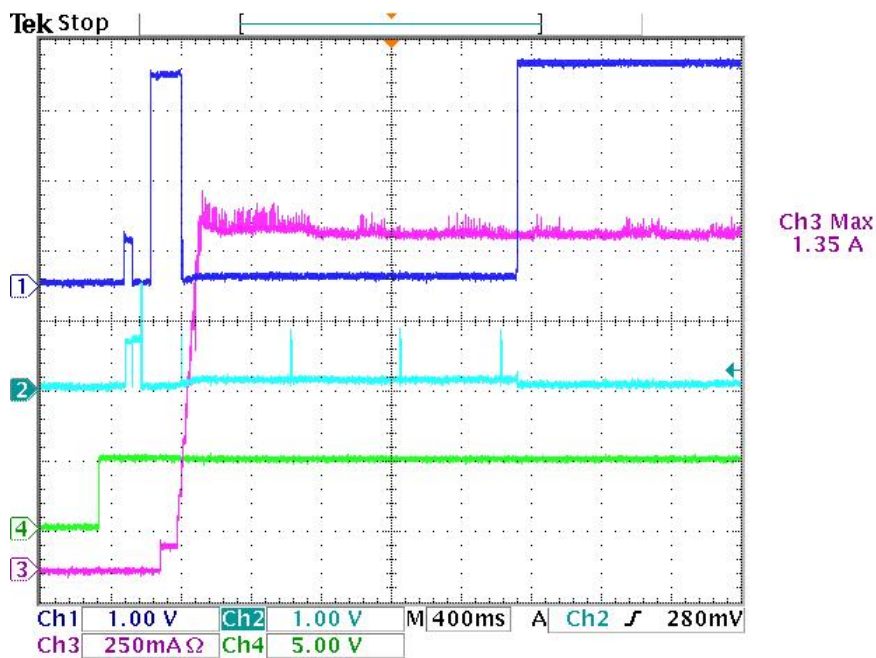
Figure 2. TPS25810 and TPS2544 (CDP Mode) Test With iPhone6, With Type C-to-B Dongle Connected to Device, Then Plug in the Host
