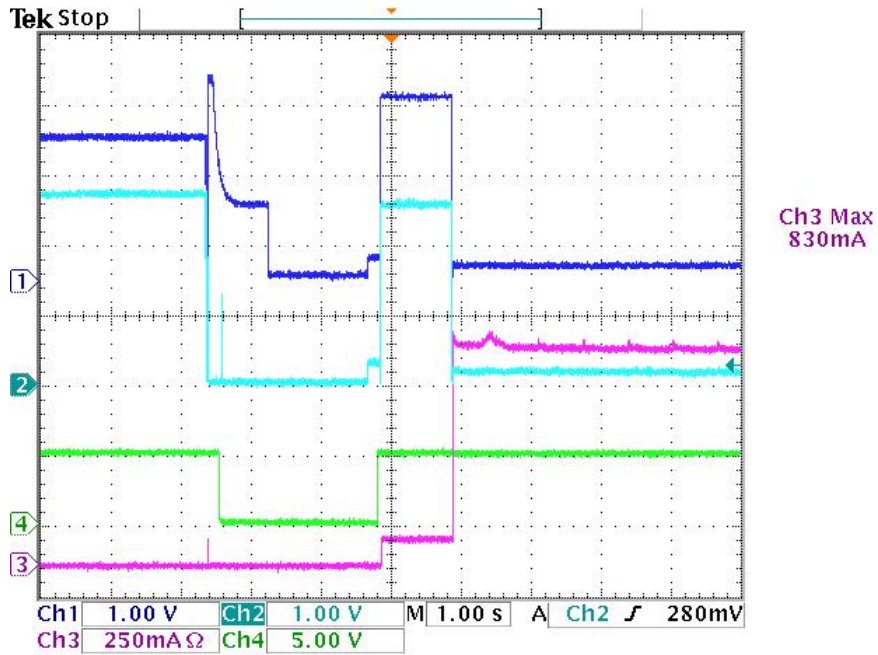
Figure 13. TPS25810 and TPS2544 (DCP Auto Mode) Test With Bold 9000, With Type C-to-B Dongle Connected to Host Then Plug In Device
