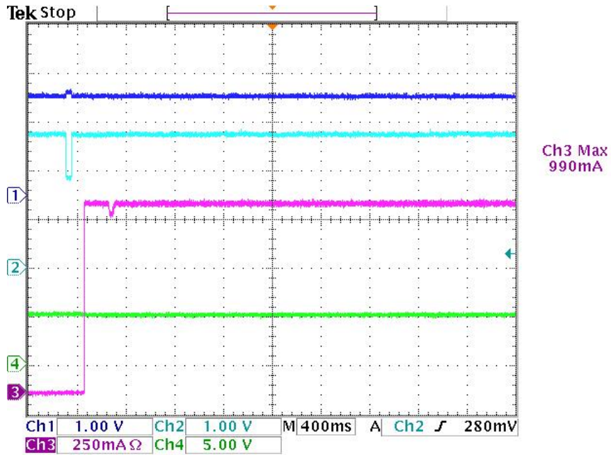
CH1: D+, CH2: D-, CH3: I OUT , CH4: V OUT Figure 9. TPS25810 and TPS2544 (DCP Auto Mode) Test With Galaxy S6, With Type C-to-B Dongle Connected to Host Then Plug In Device
