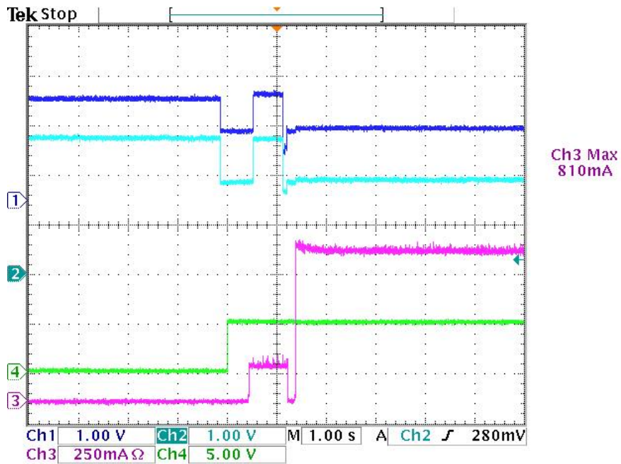
CH1: D+, CH2: D-, CH3: I OUT , CH4: V OUT Figure 10. TPS25810 and TPS2544 (DCP Auto Mode) Test With HTC Sense, With Type C-to-B Dongle Connected to Device Then Plug In Host
