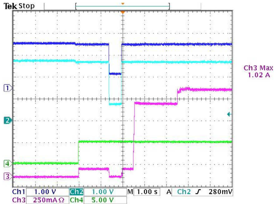
Figure 6. TPS25810 and TPS2544 (DCP Auto Mode) Test With iPhone6, With Type C-to-B Dongle Connected to Device Then Plug In Host
