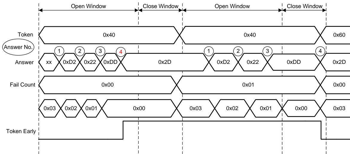
Figure 6. Out-of-Timing Window Timing Diagram
