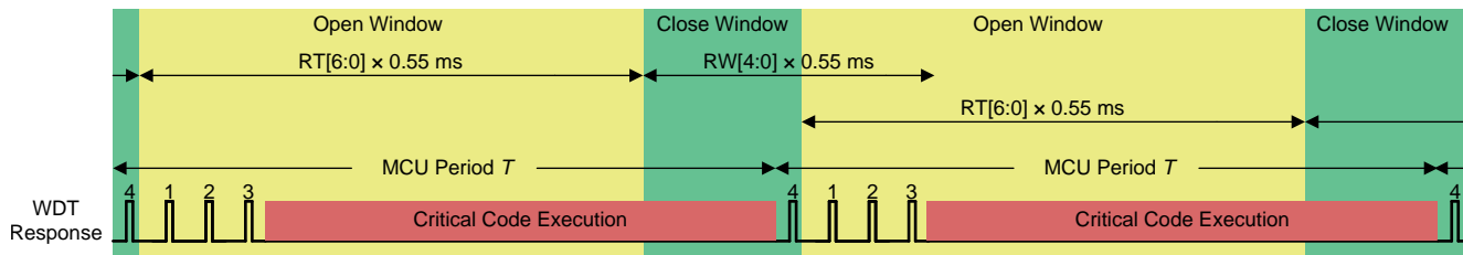
Figure 9. Watchdog Response Scheduling
