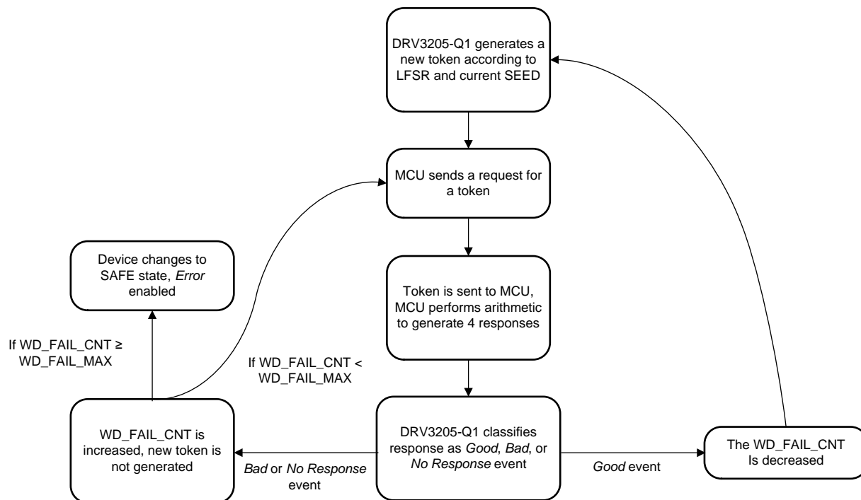
Figure 2. Simplified Watchdog-Timer Flow Chart
