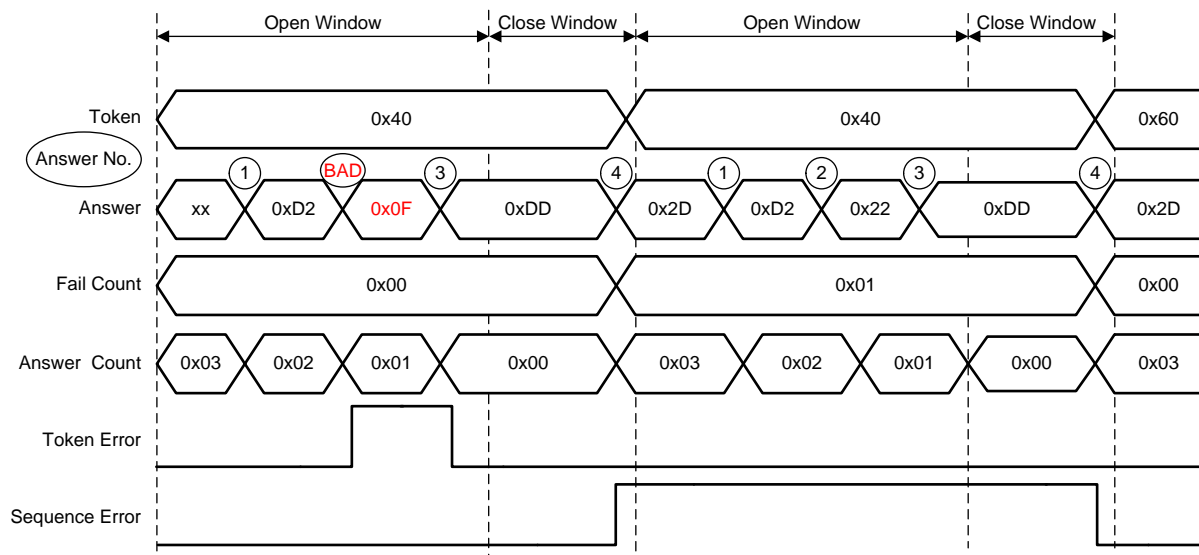
Figure 4. Incorrect Answer-Value Timing Diagram
