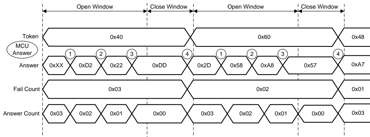
Figure 3. Watchdog-Timer Good Event
