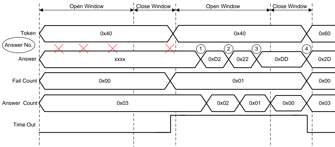
Figure 7. WDT No Response Event
