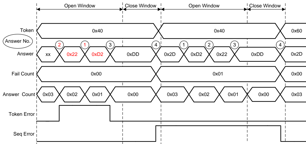
Figure 5. Incorrect Answer Sequence Timing Diagram
