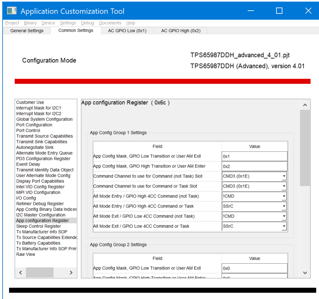
Figure 4. App Config Group 1 Settings
