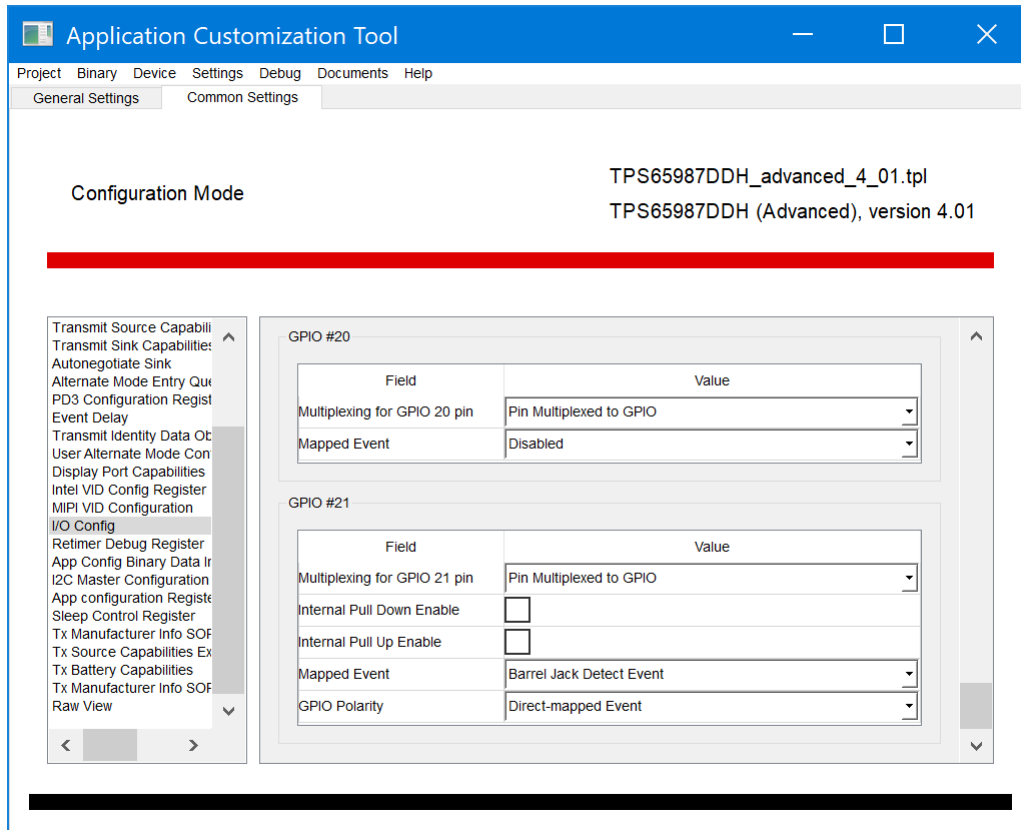
Figure 9. GPIO 21 Settings
