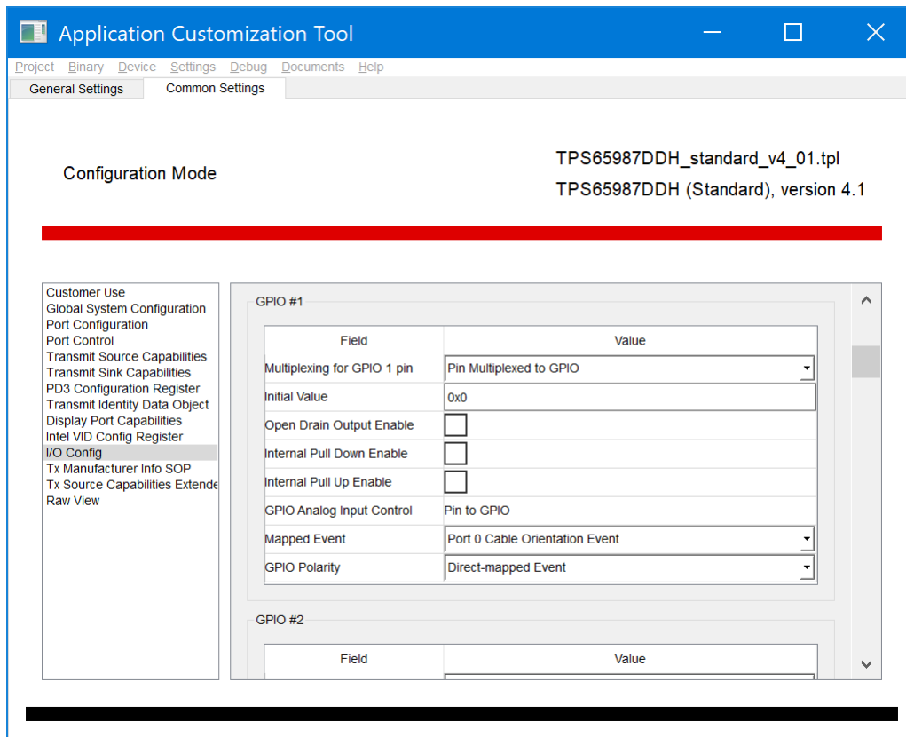
Figure 2. Template with GPIO Events Mapped for TPS65987D EVM
