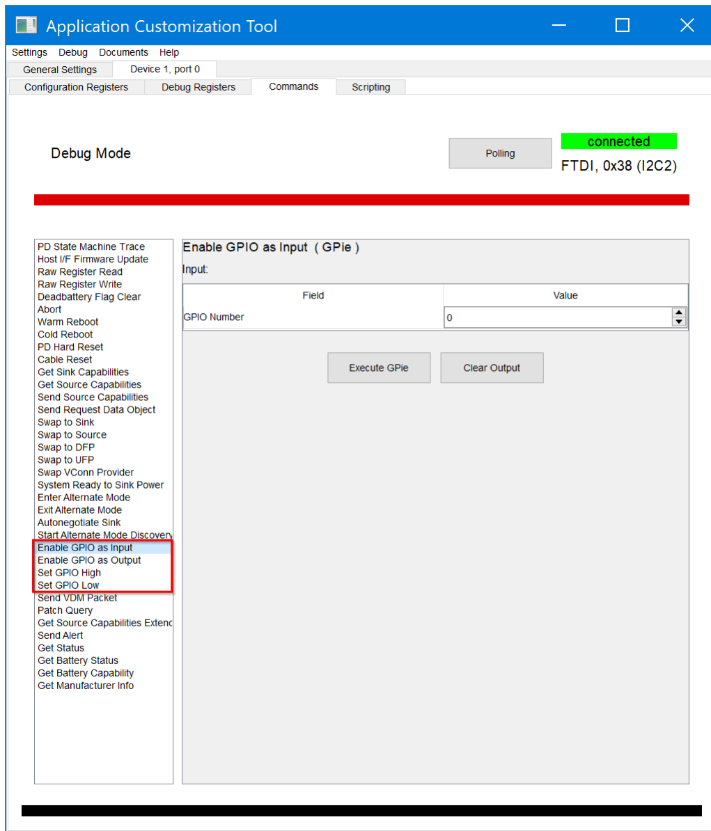
Figure 14. 4CC Commands in TPS6598x Application Customization Tool
