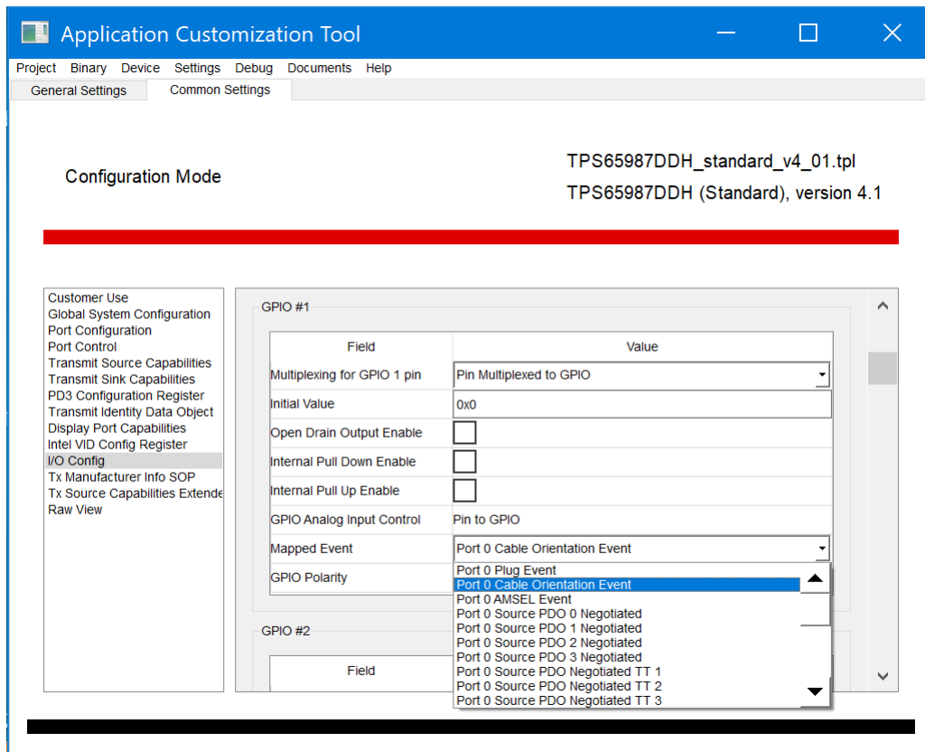
Figure 1. Mapping a GPIO Event using TPS6598x Application Customization Tool
