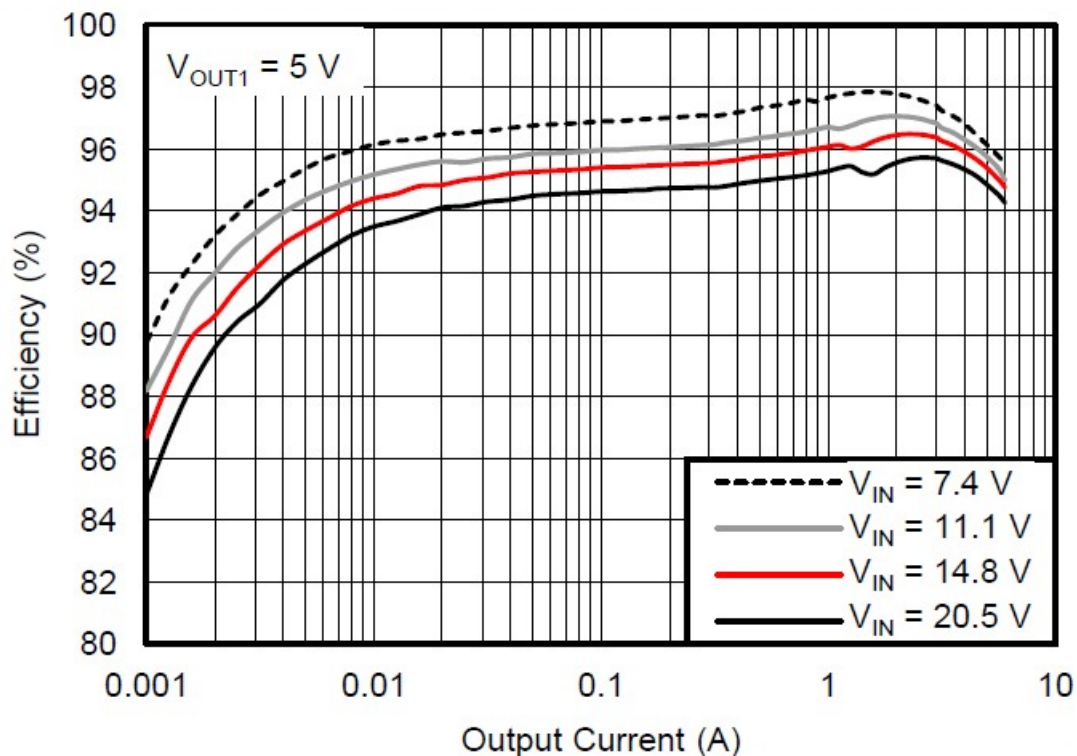
Figure 1. TPS51285A Efficiency plot with Eco-Mode™ and ULQ™
