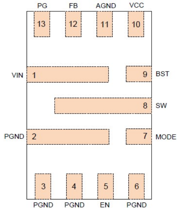
Figure 4. TPS566335 2x3mm QFN package view
