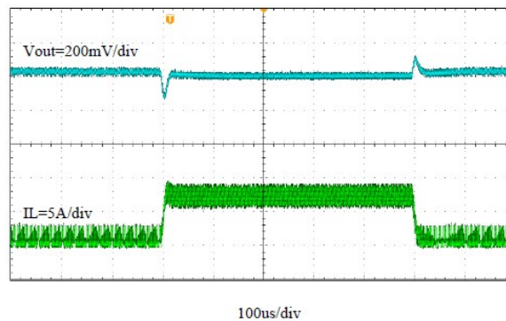
Figure 2. TPS51395 Load Transient Waveform
