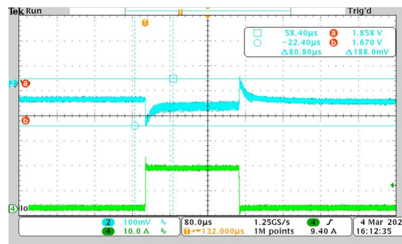
Figure 3. TPS51215A Load Transient Waveform
