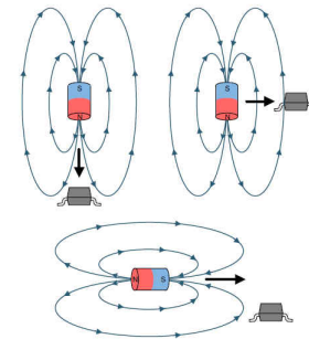
Figure 2. Correct magnetic field detection for traditional sensors
