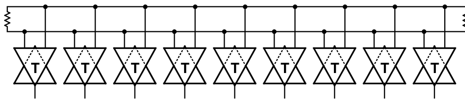
Figure 4. Common Bus Configuration: Multi-Point
