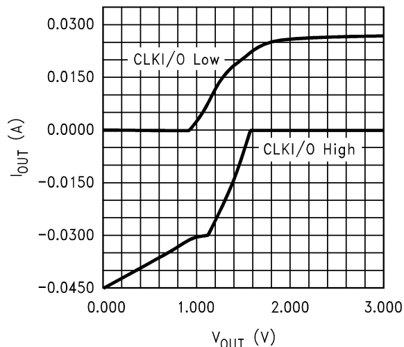
Figure 8. Voltage vs Current for CLKI/O Signals (simulation): DS92CK16 Sim of V vs I for CLKI/O High and Low Cases, V_{CC} = 3.3\text{ V} , T_A = 25^\circ\text{C}
