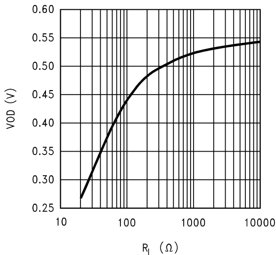
Figure 9. VOD vs R_L : DS92CK16 CLKI/O VOD vs R_L , V_{CC} = 3.3\text{ V} , T_A = 25^\circ\text{C}
