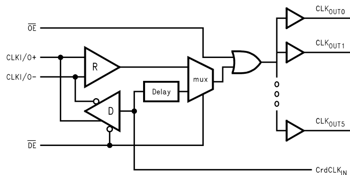
Figure 1. Block Diagram of DS92CK16
