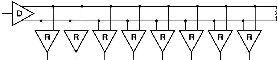
Figure 3. Common Bus Configuration: Multi-Drop
