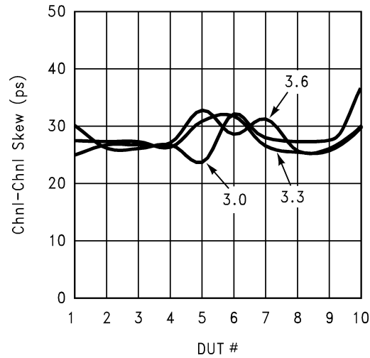
Figure 12. Receiver Channel to Channel Skew at 85°C: DS92CK16 Ave Skew at 85°C
