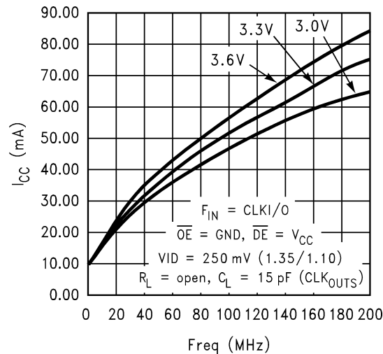
Figure 13. Typical I_{CC} vs Frequency. Input is CLKI/O: DS92CK16 I_{CC} vs Freq. Receiver Mode
