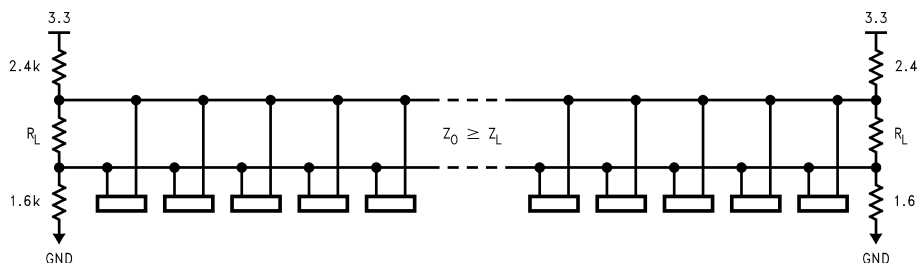
Figure 5. Typical Failsafe Biasing Scheme
