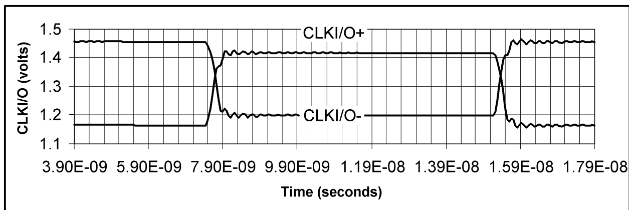
Figure 6. Backplane Termination and Failsafe Biasing: Failsafe Loading Simulation—DS92CK16 75Ω Bus With 1.2 kΩ Pull Up and 800 Ω Pull Down
