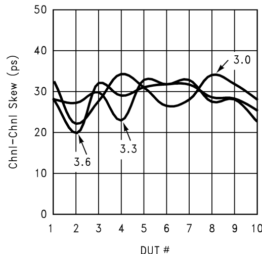
Figure 11. Receiver Channel to Channel Skew at 25°C: DS92CK16 Ave Skew at 25°C
