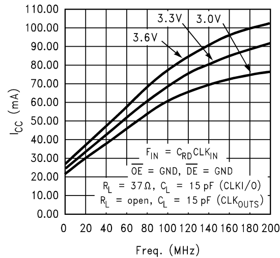
Figure 14. I CC vs Frequency With the C RD CLK in as the Input, and CLKI/O, CLK OUT Pins Switching: DS92CK16 I CC vs Freq. CLKI/O and CLK OUT Switching
