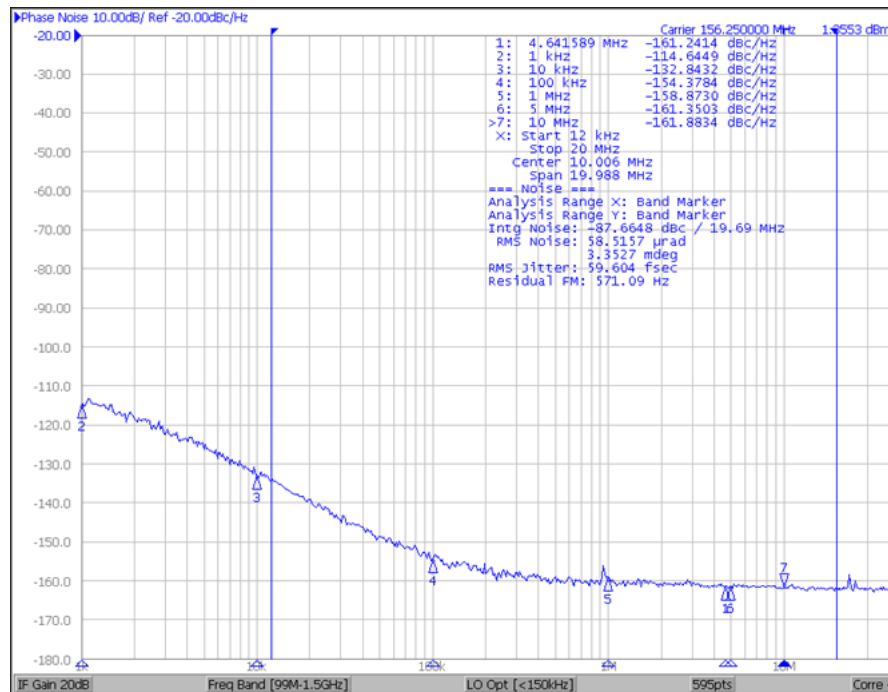
Figure 2. 156.25-MHz LVPECL Phase Noise of LMK05318
